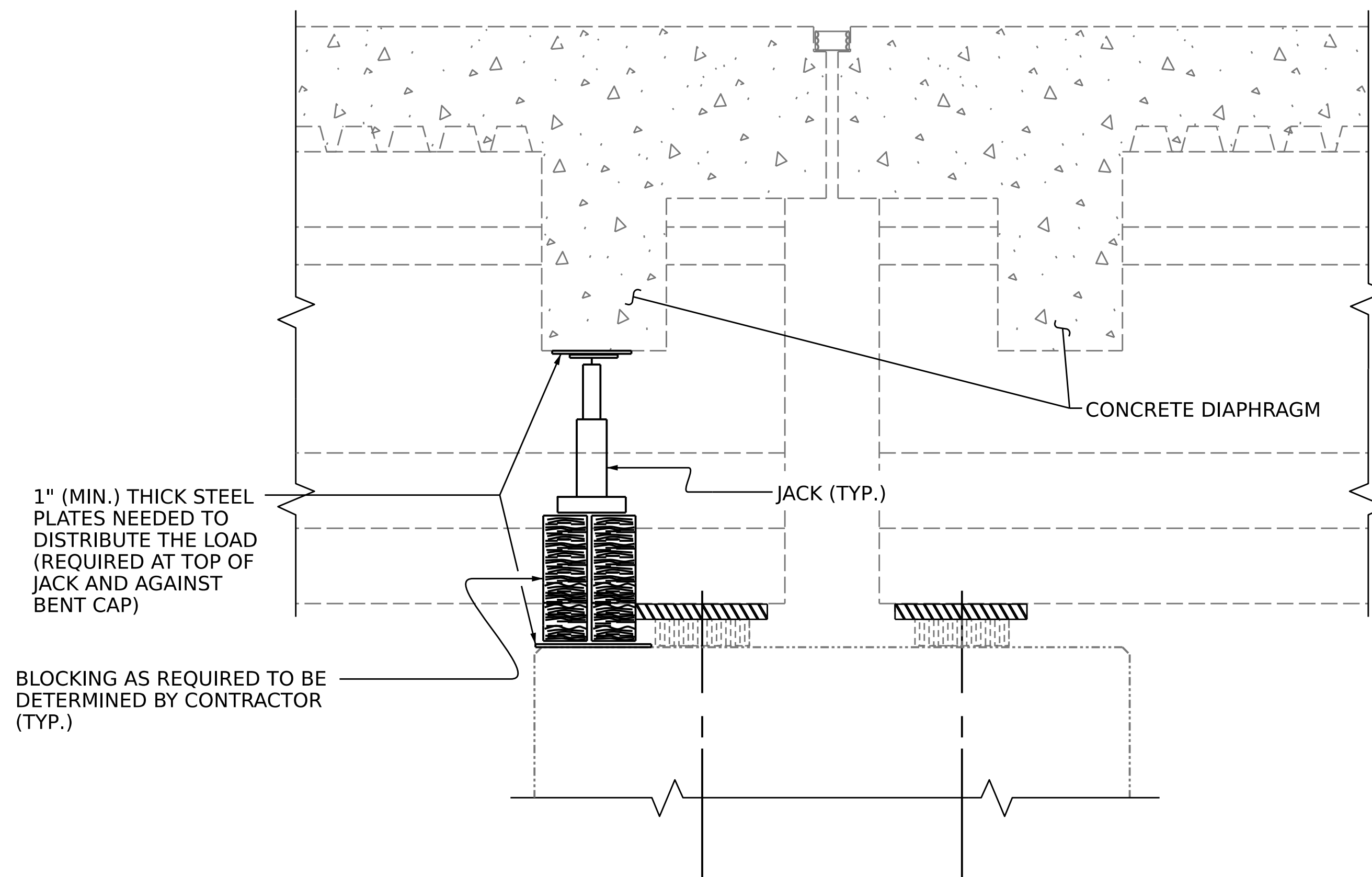
SECTION THRU DIAPHRAGM
