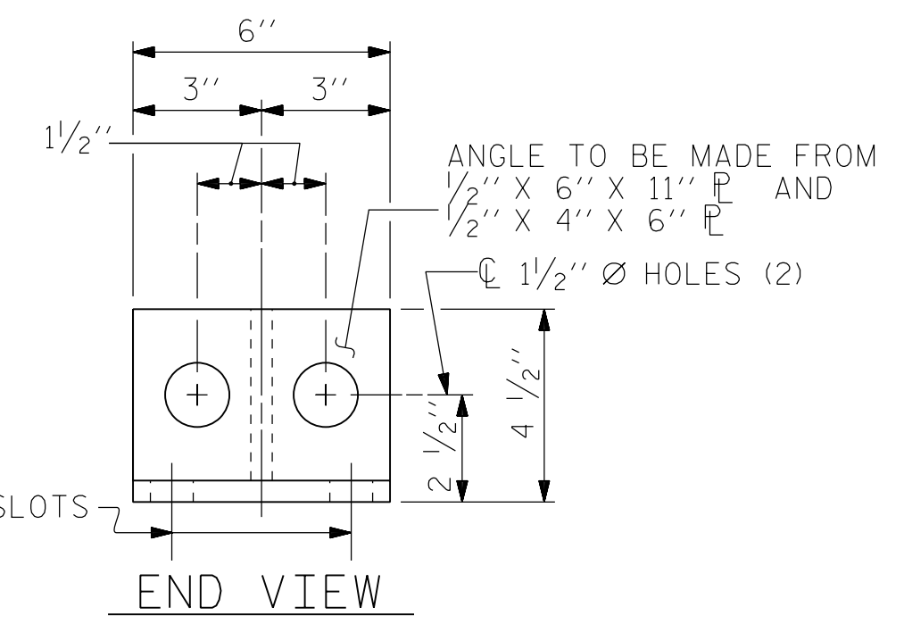
DETAILS FOR ATTACHMENT BRACKET (BOTTOM RAIL ONLY)
