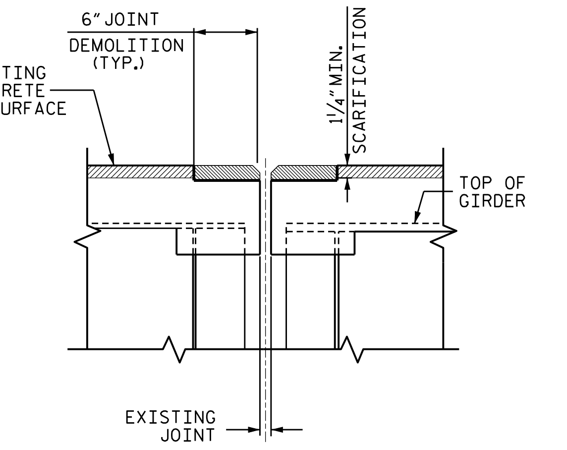
MINIMUM EXISTING JOINT DEMOLITION & SCARIFICATION
