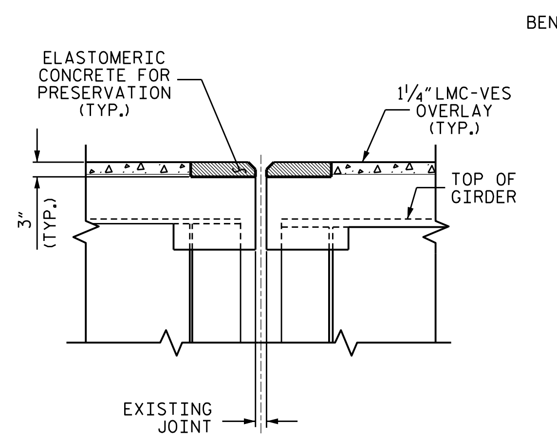
PROPOSED PRE-SAWED JOINT
