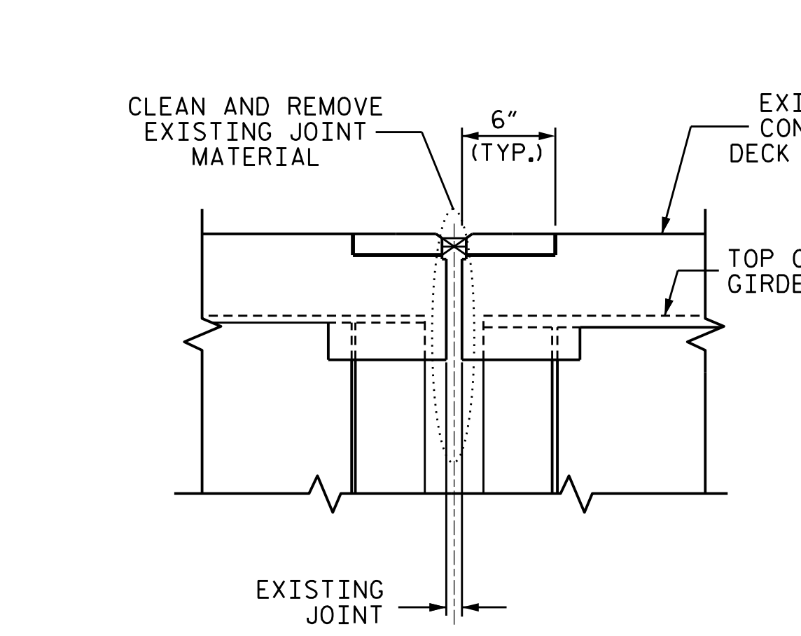
EXISTING JOINT
