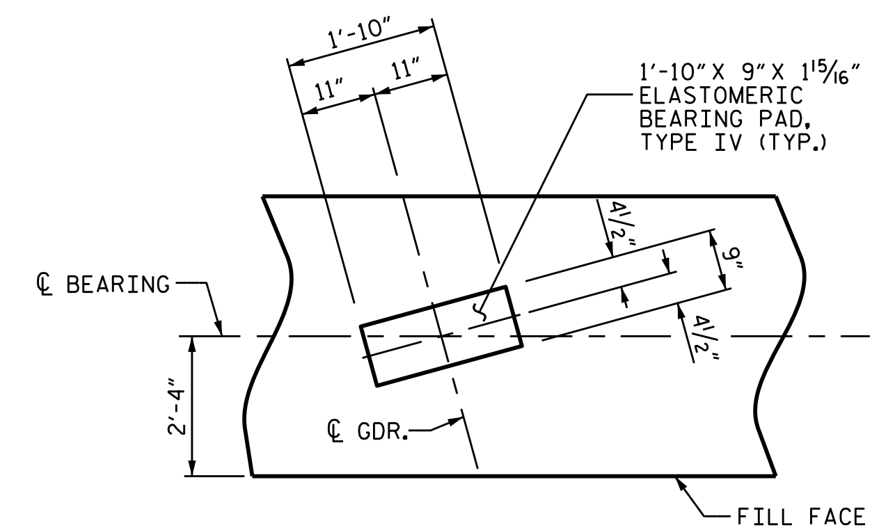
DETAIL "A"
