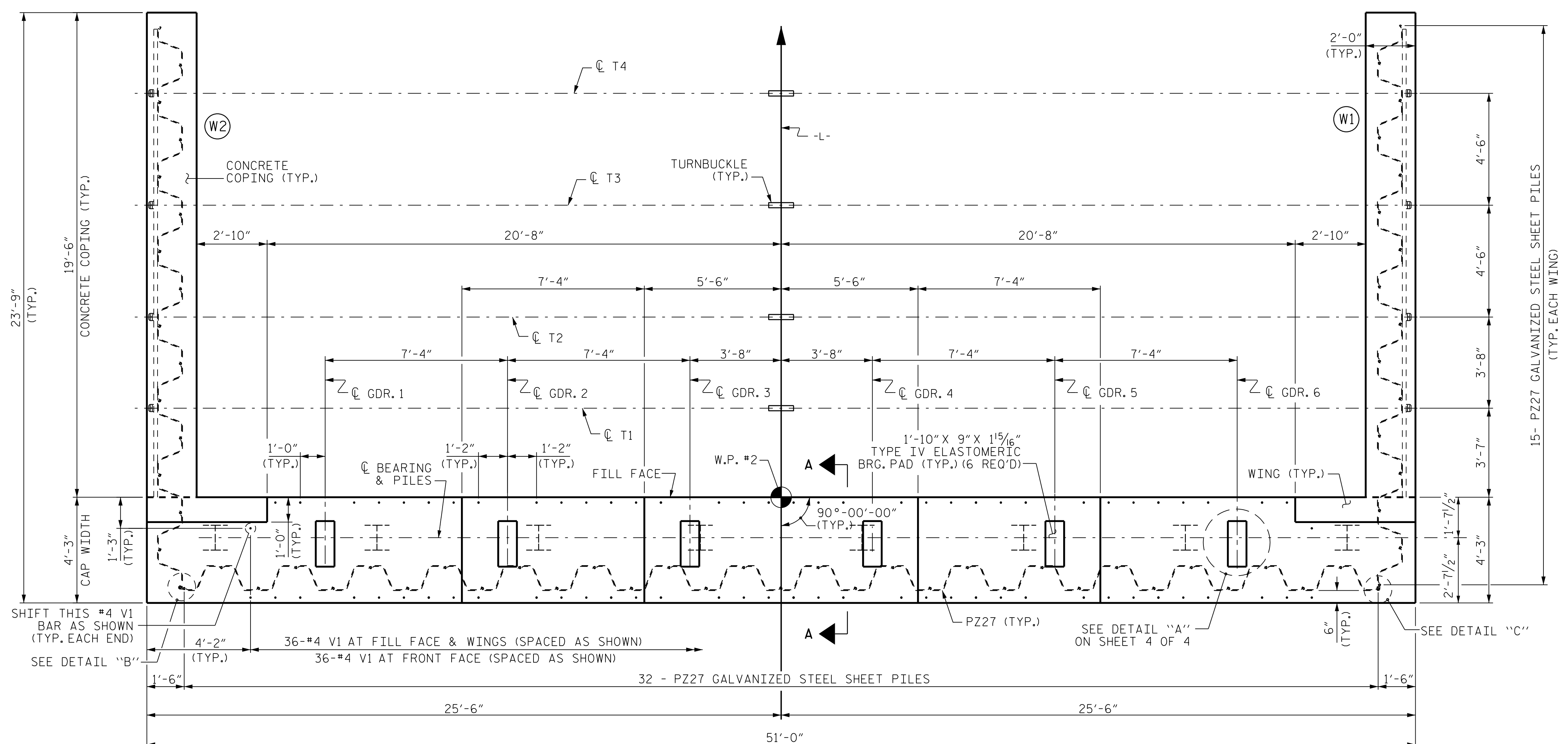
PLAN
