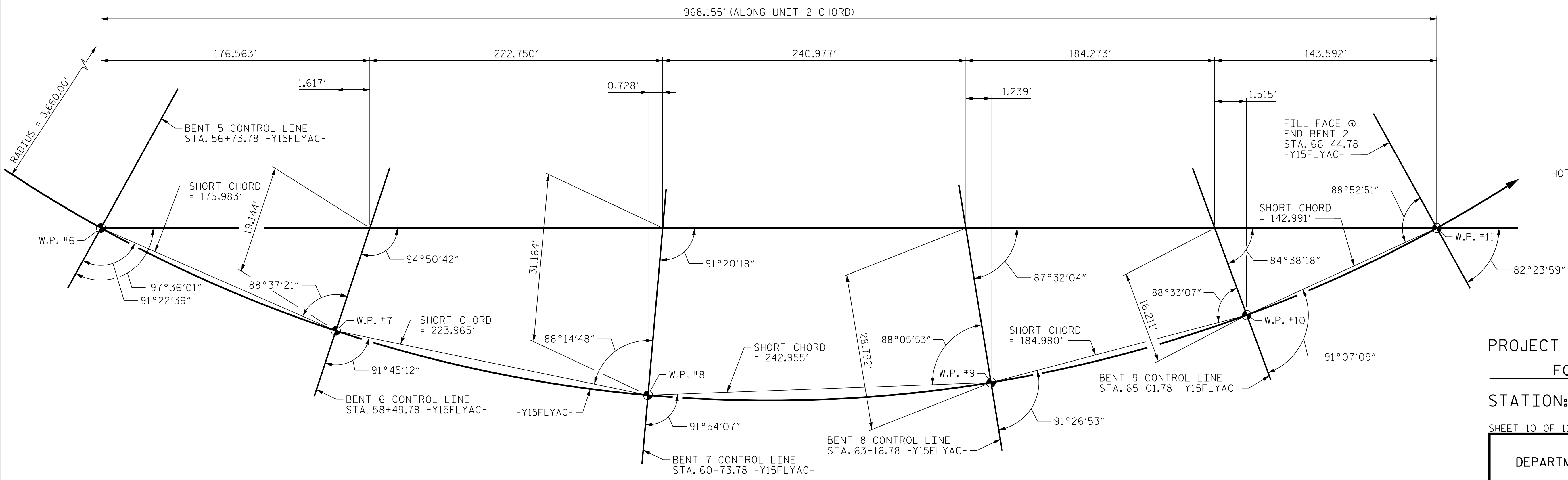
UNIT 2 CHORD LAYOUT ALL BENTS ARE RADIAL TO -Y15FLYAC-
