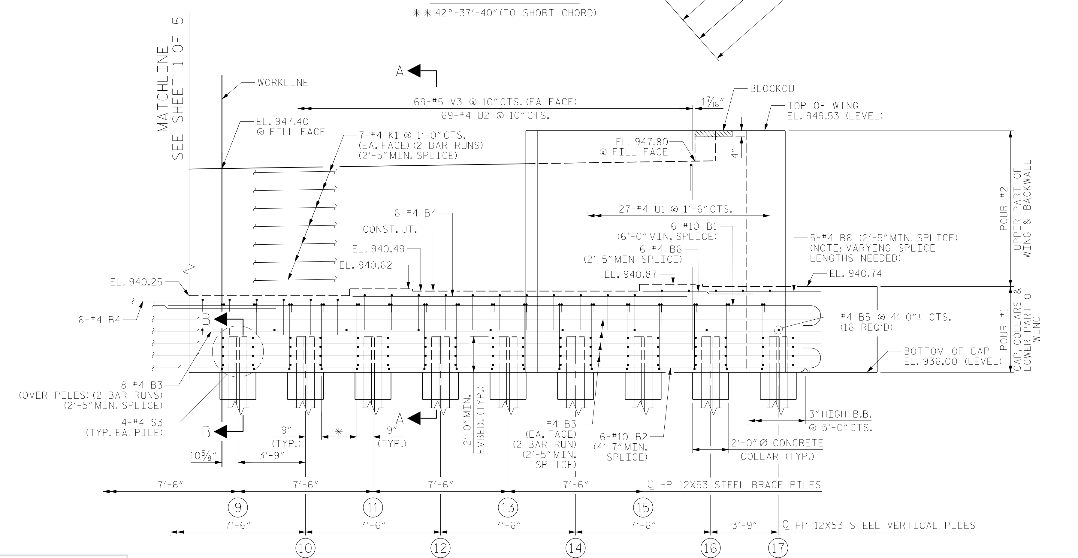
PARTIAL ELEVATION * 4-#5 S1 & #5 S2 @ 9\"/>
