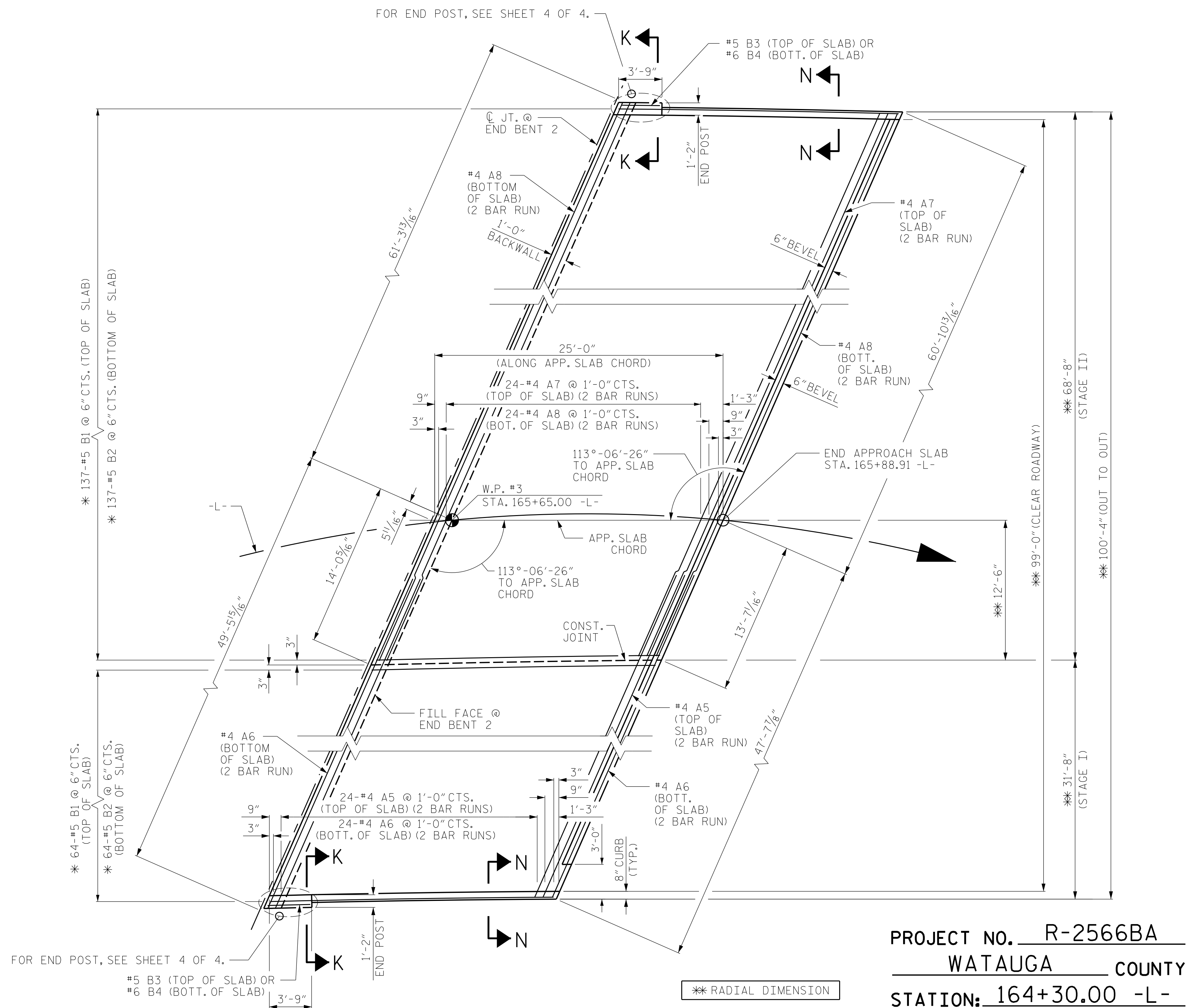
PLAN OF APPROACH SLAB @ END BENT 2
