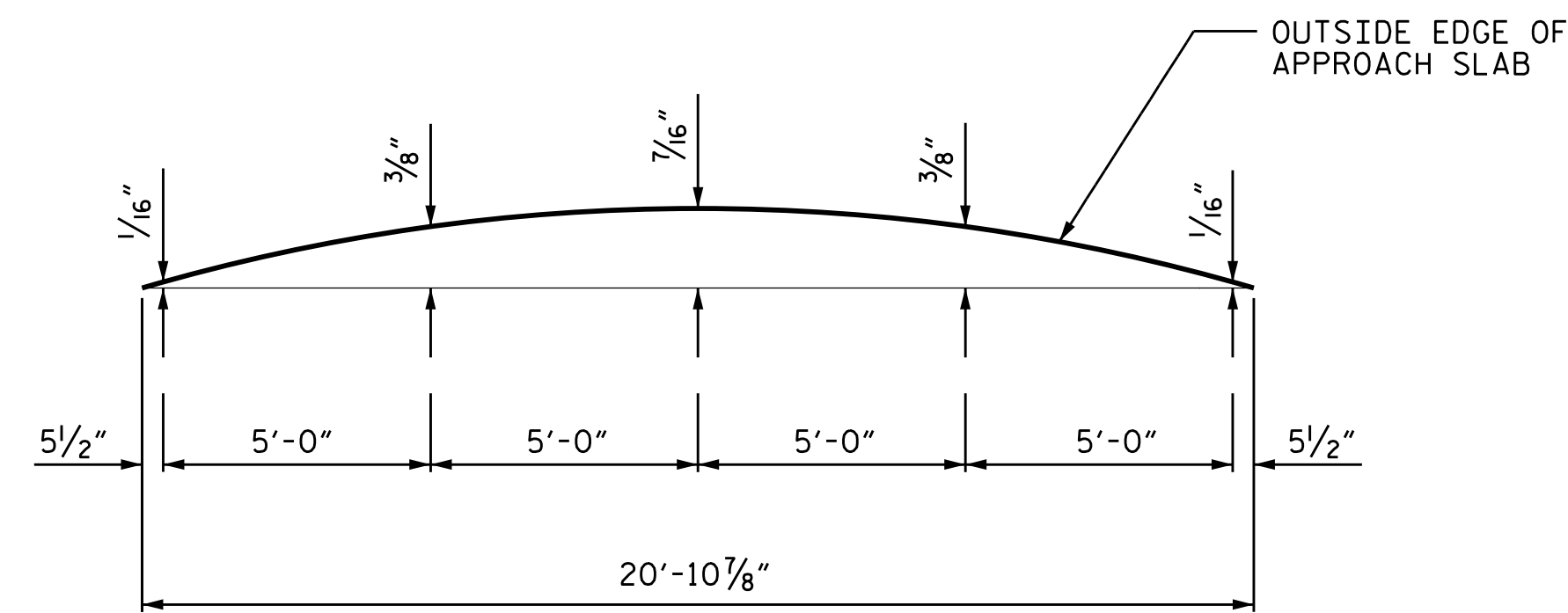
ARC OFFSETS LEFT SIDE
