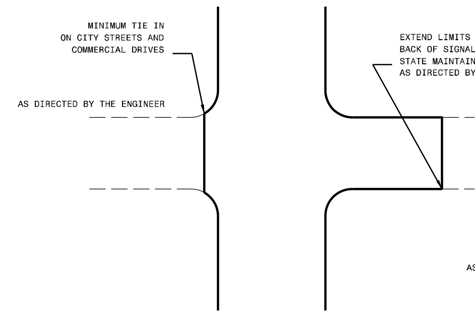
DETAIL OF PROJECT LIMITS AT SIGNALIZED Y LINES
