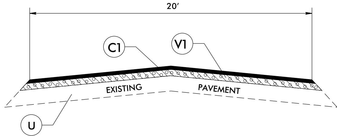
TYPICAL SECTION NO. 13
