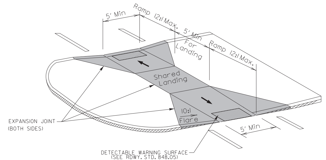
MEDIAN ISLAND CURB RAMPS TYPE 8
