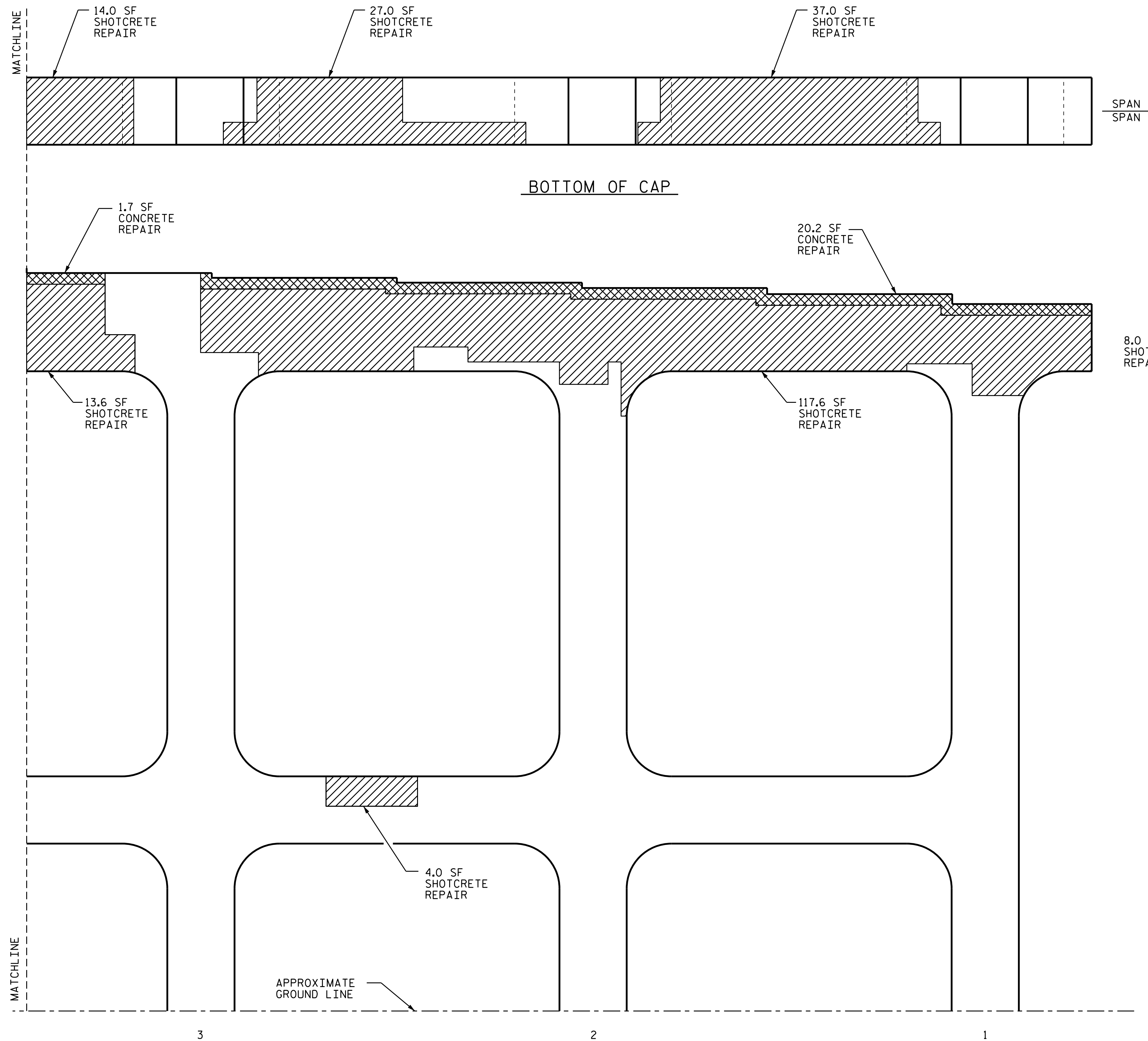
ELEVATION BENT 11
