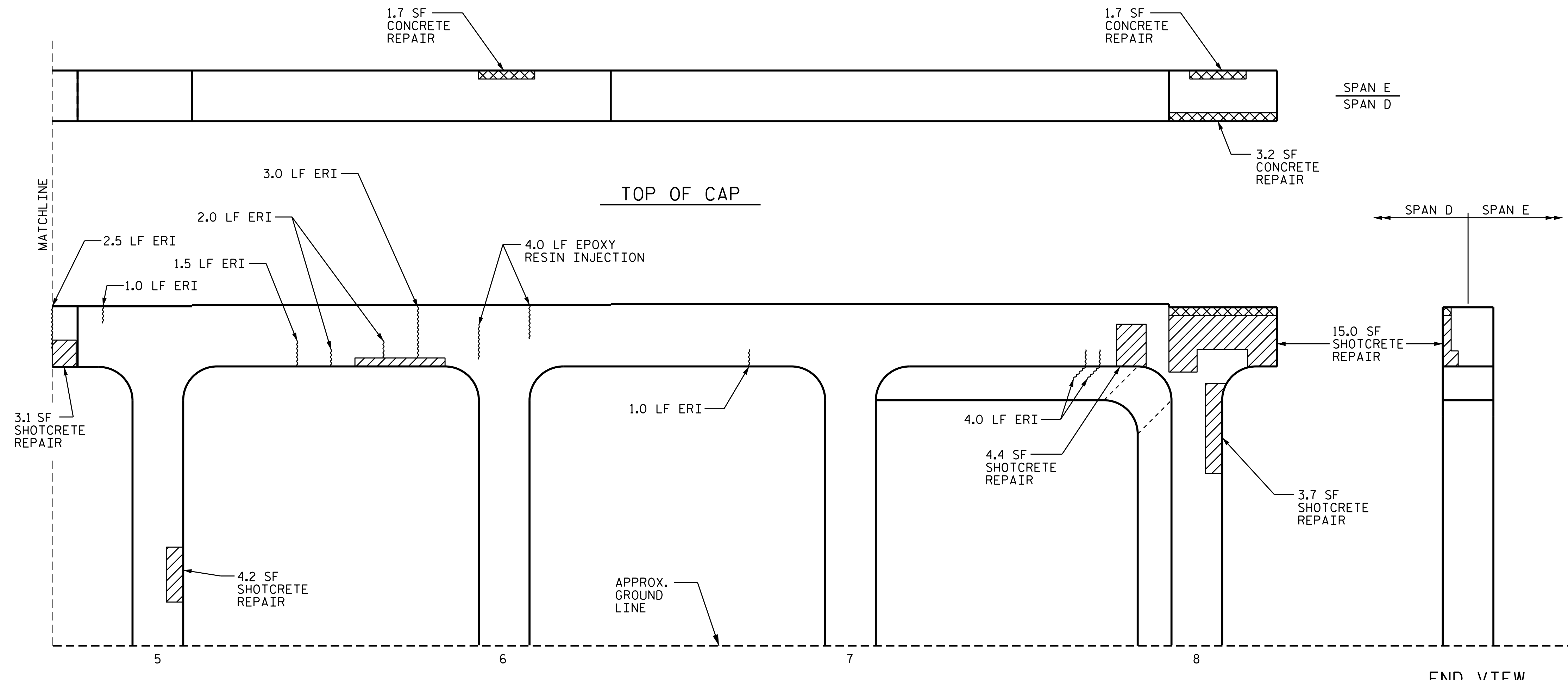
ELEVATION BENT 4
