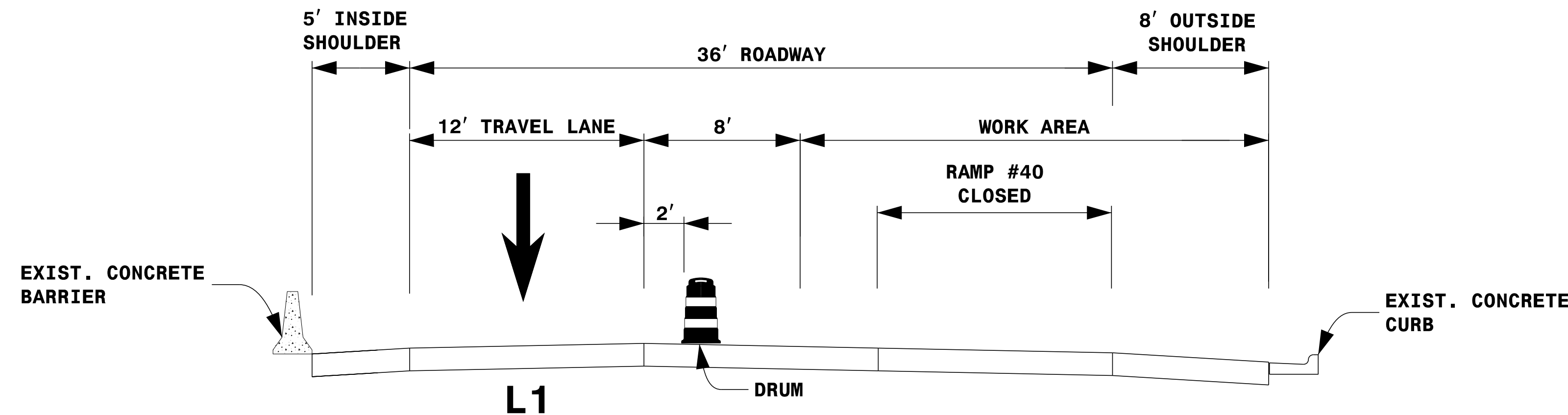
TYPICAL SECTION SECTION 13E SOUTHBOUND
