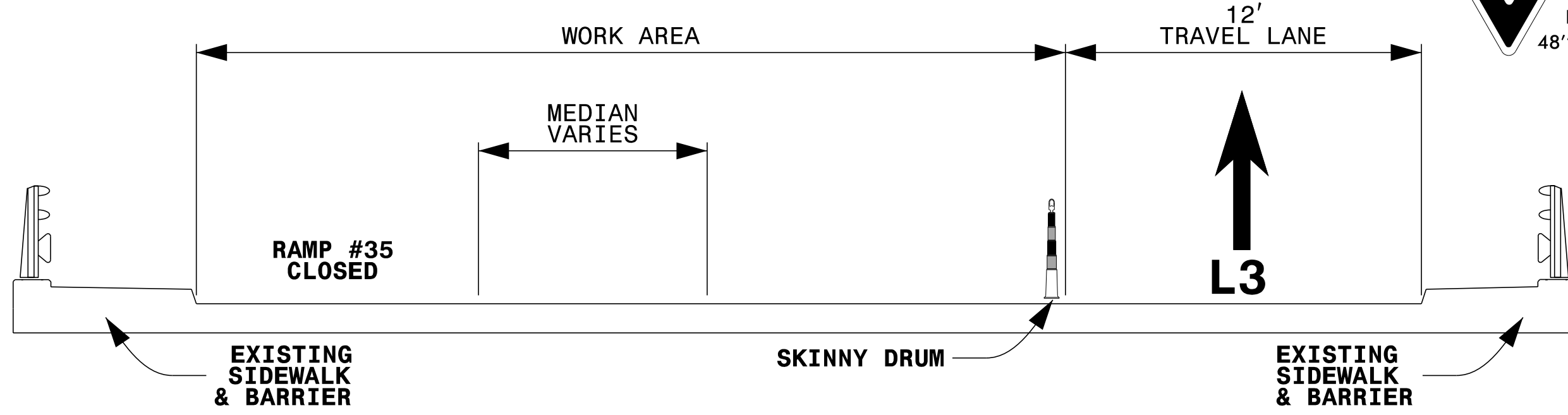
TYPICAL SECTION BRIDGE #138 NORTHBOUND (INSIDE LANES)
