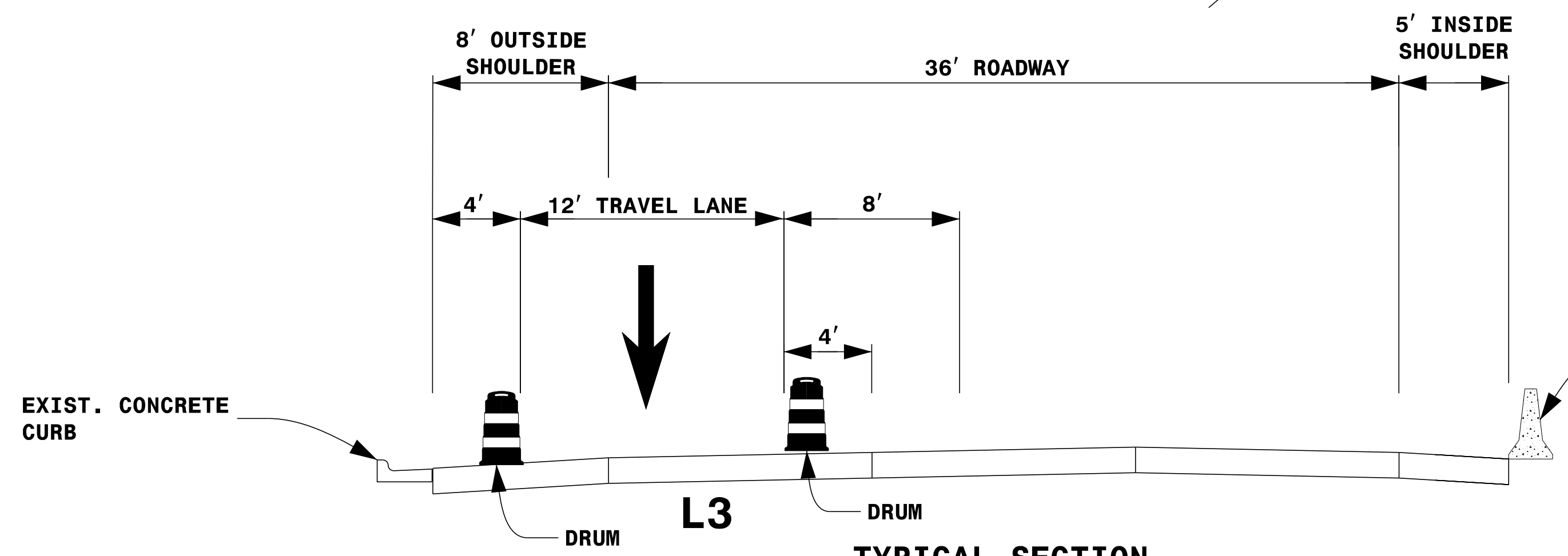
TYPICAL SECTION BRIDGE #328 SOUTHBOUND
