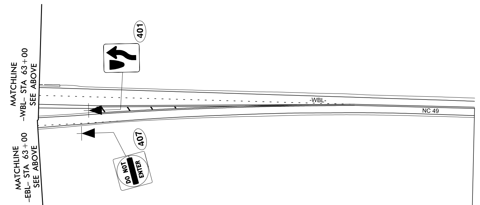
END PAVEMENT MARKING PROJECT B-4626 -EBL- STA. 70+31 TIE TO EXISTING
