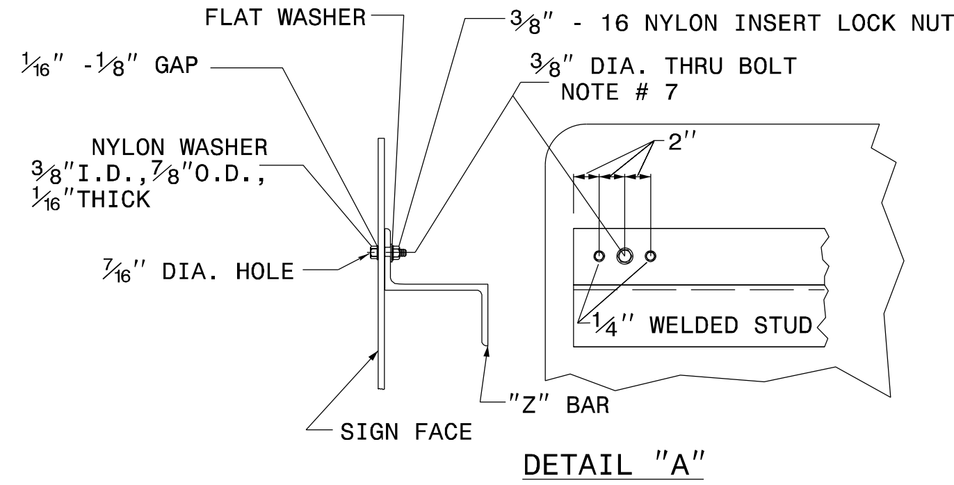
DETAIL "A"
