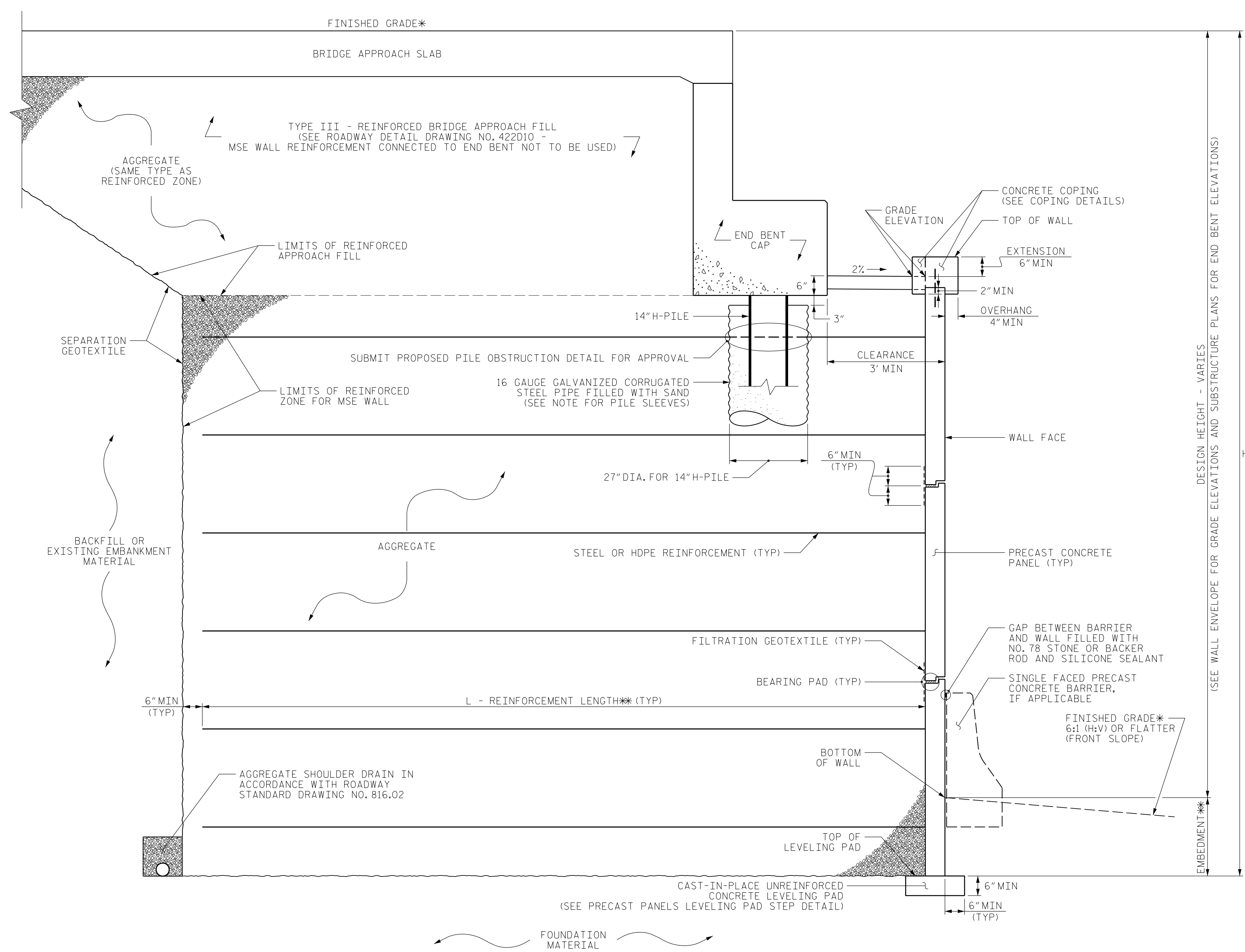
MSE ABUTMENT WALL WITH PRECAST PANELS - TYPICAL SECTION -RW3- 13+91.09 TO 15+09.20
