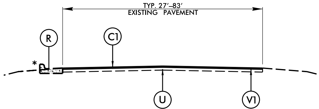
TYPICAL SECTION 2 2" MILL, FILL AND RESURFACE S9.5C MAP NOS. 3-6
