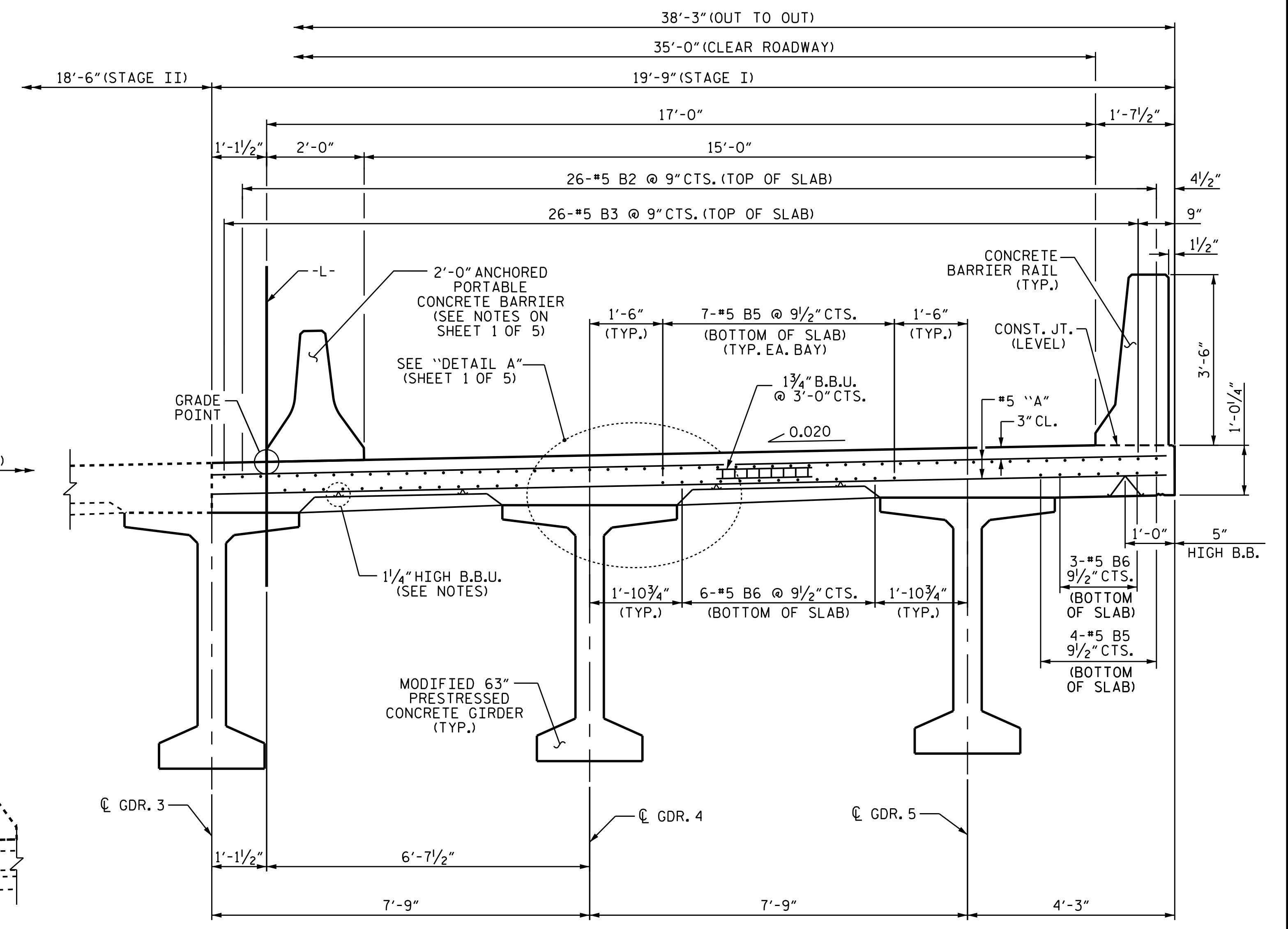
LINK SLAB AT BENT (STAGE I)
