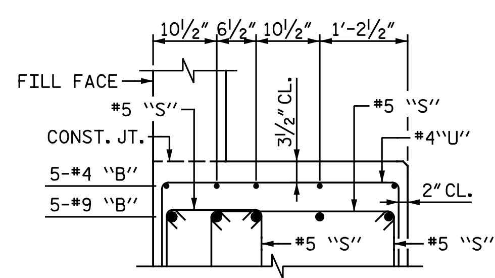
BEAM SEAT DETAILS
