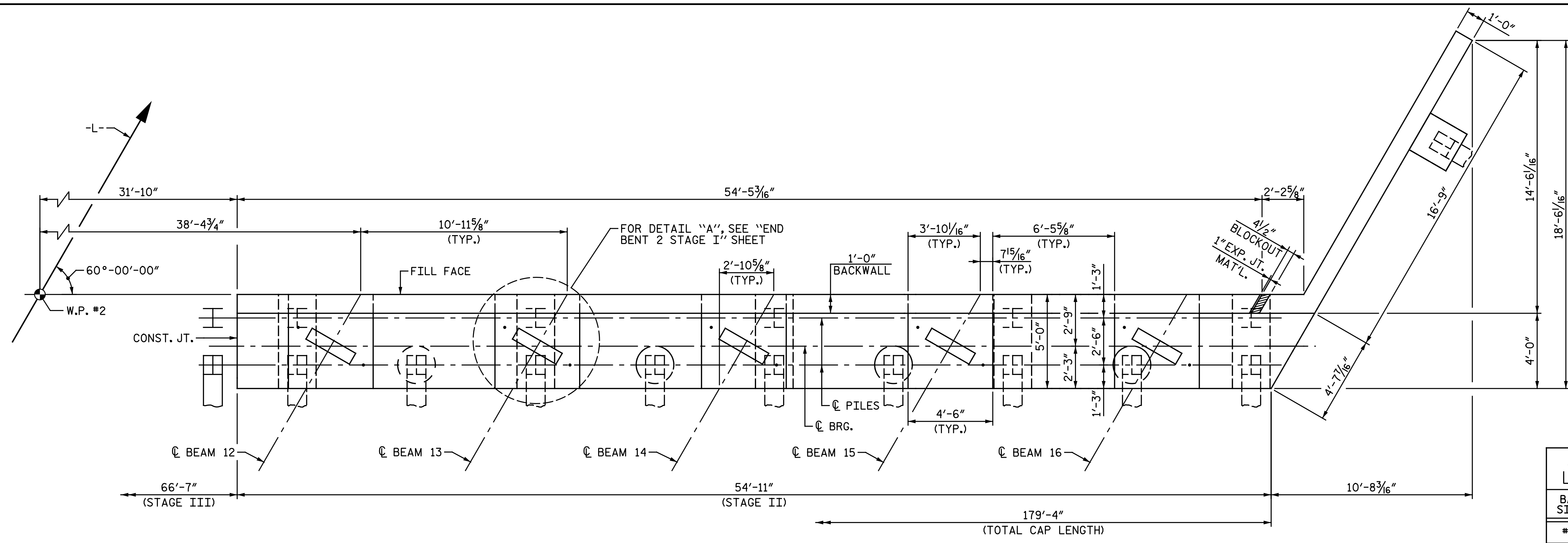
PLAN - STAGE II FOR LOCATION OF BRACE PILE IN WING, SEE "GENERAL DRAWING" SHEET 3 OF 4.
