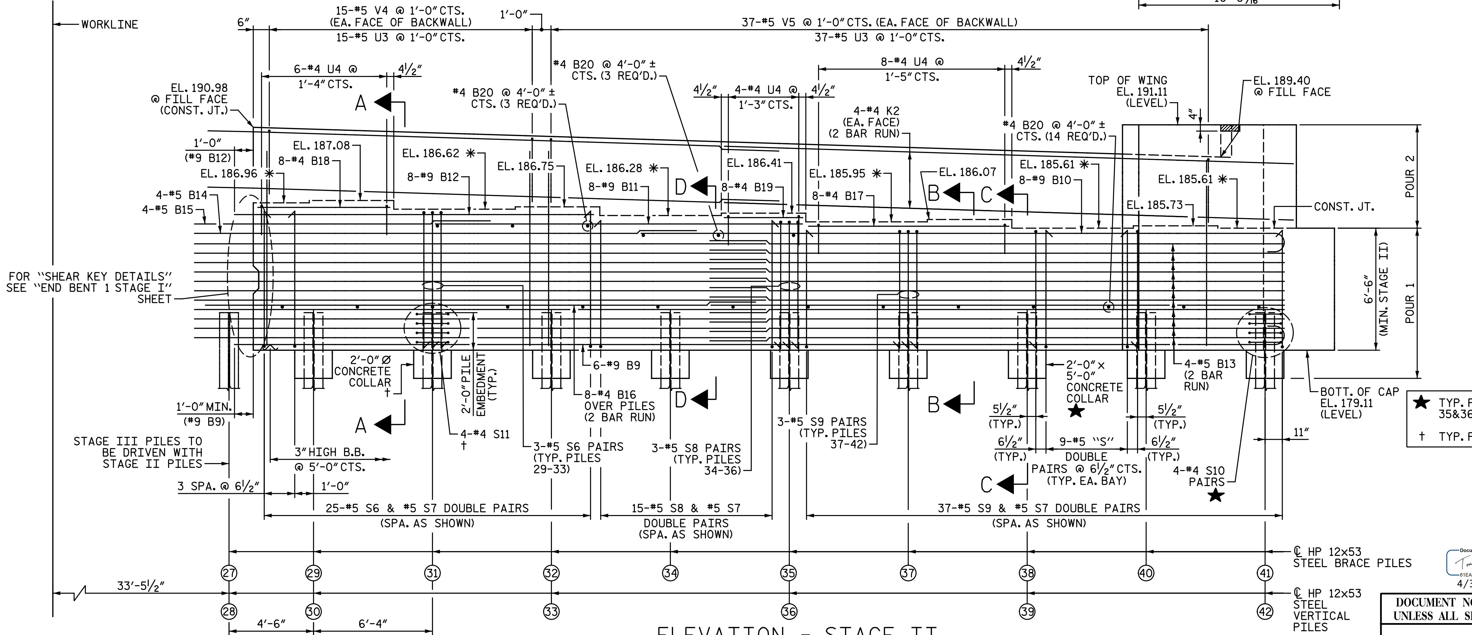
ELEVATION - STAGE II
