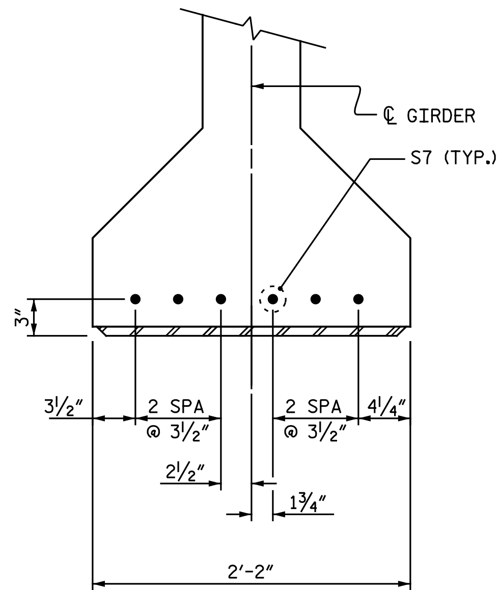
DETAIL "A"
