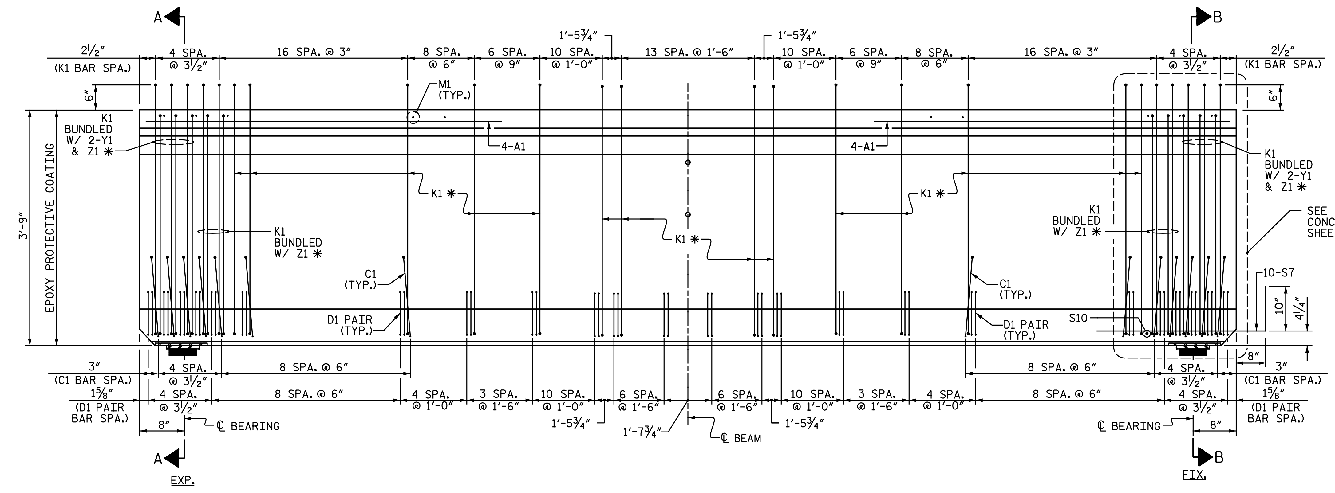
ELEVATION OF BEAM FOR "SECTION A-A" & "SECTION B-B", SEE SHEET 2 OF 4
