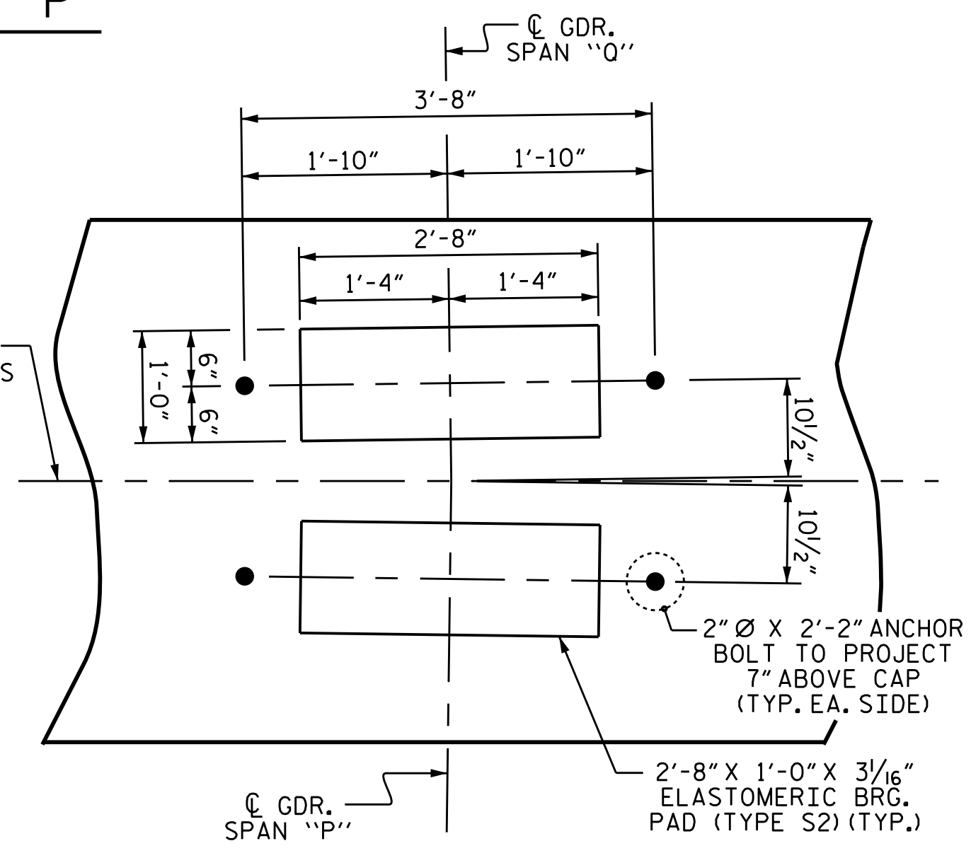
DETAIL "A" (TYP. @ EACH GDR.)
