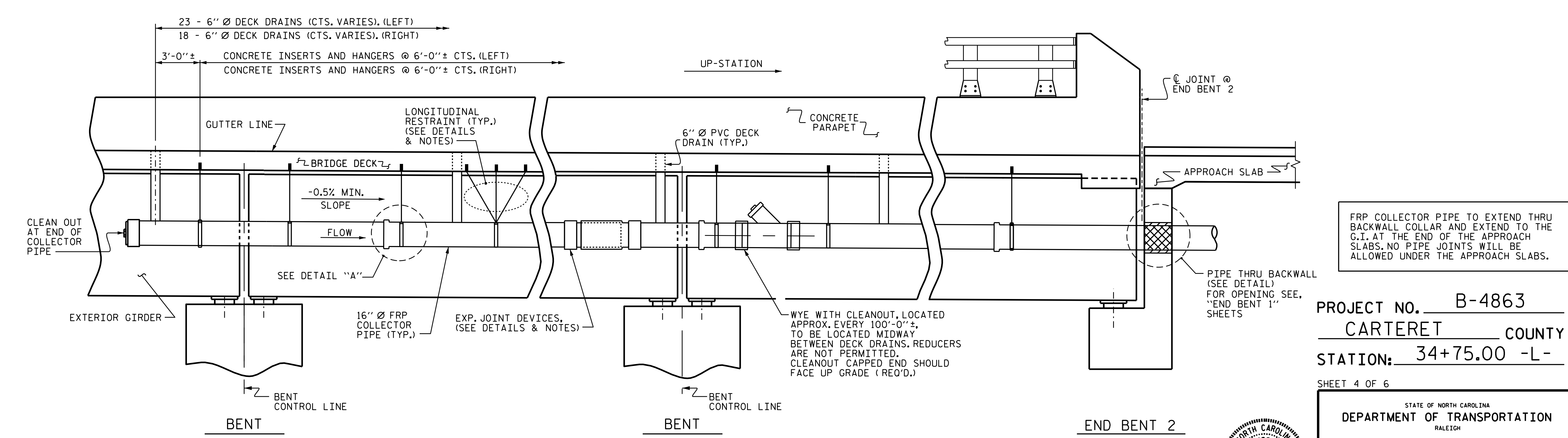
ELEVATION OF DRAINAGE SYSTEM
