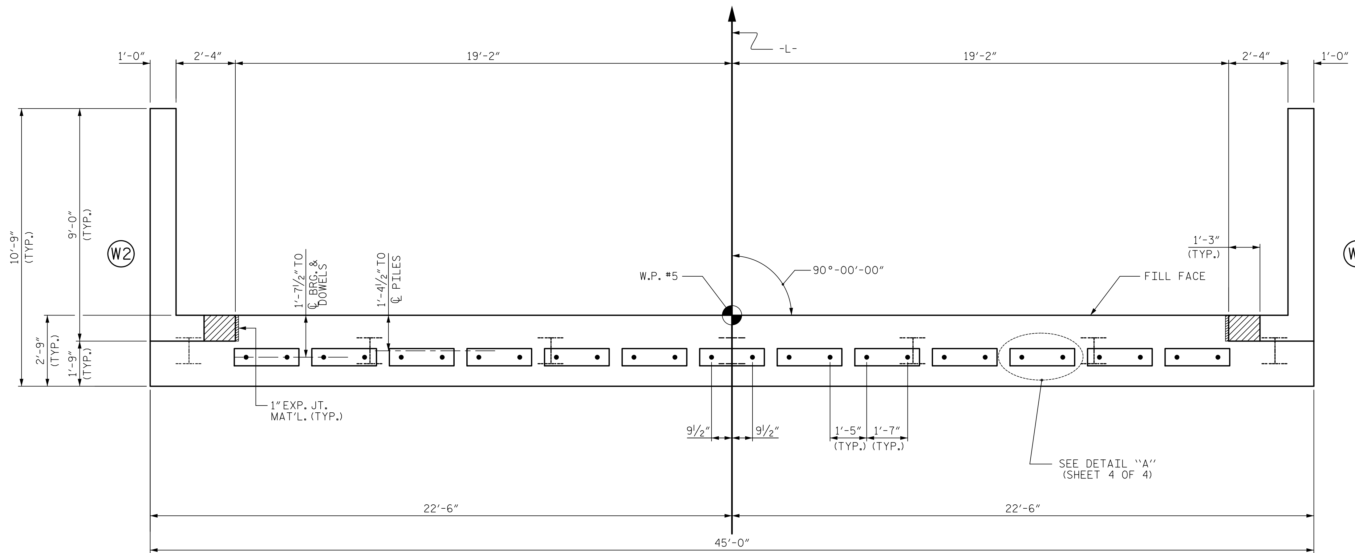
PLAN
