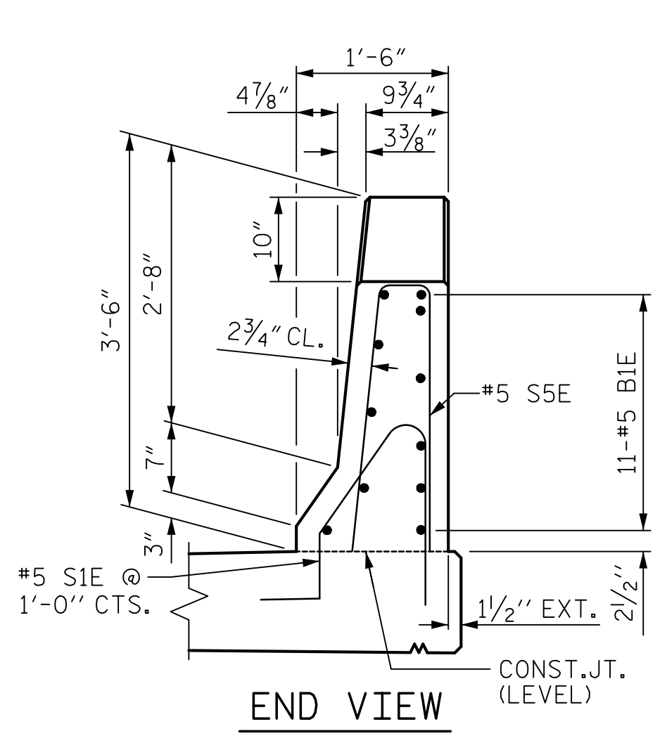
END OF RAIL DETAILS
