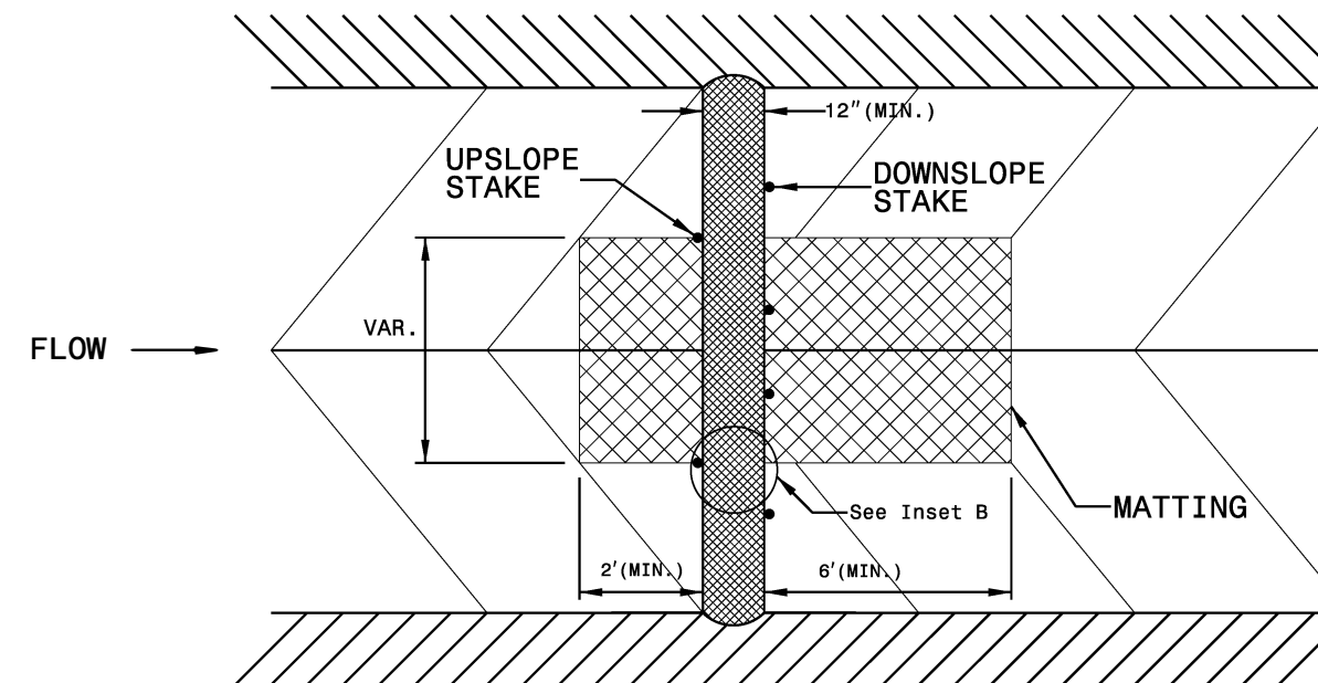
TOP VIEW
