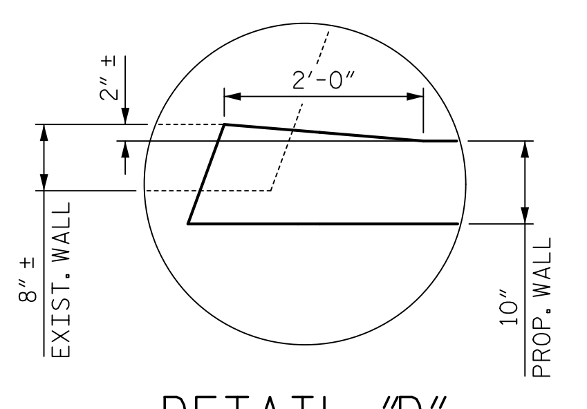
DETAIL "D"
