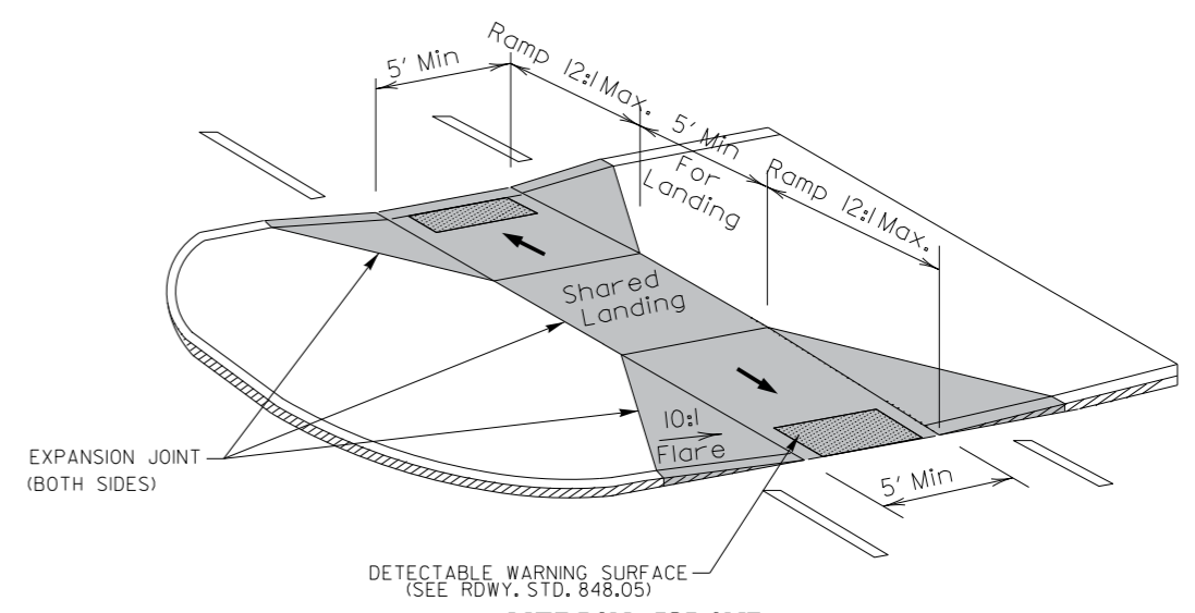
MEDIAN ISLAND TYPE 8 CURB RAMPS 1/8/2020
