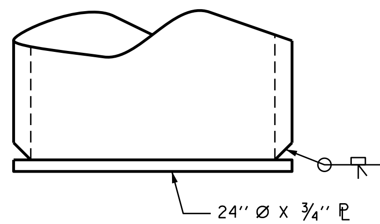
PIPE PILE PLATE DETAIL
