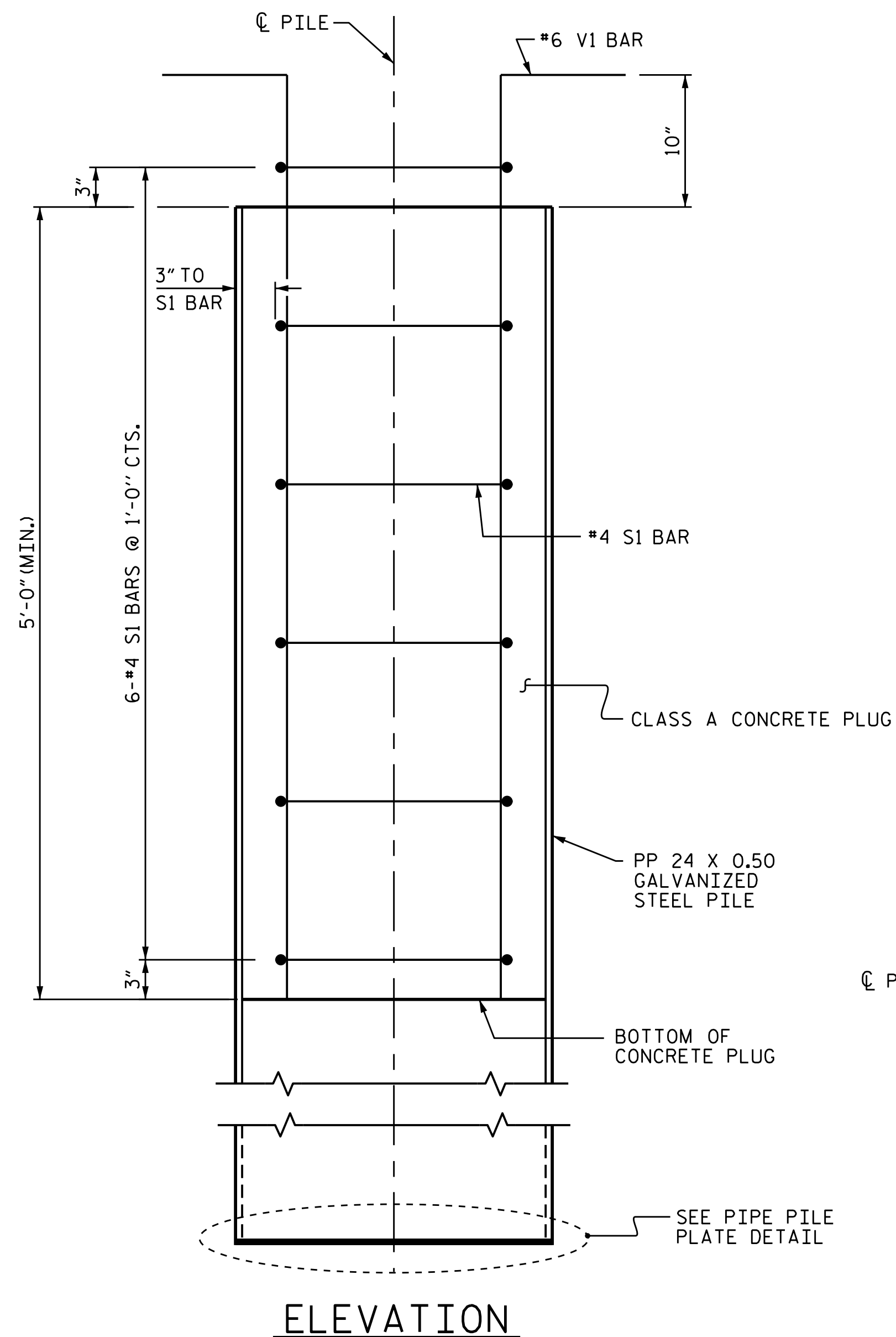
PP 24 X 0.50 GALVANIZED STEEL PILE (CLOSED ENDED)
