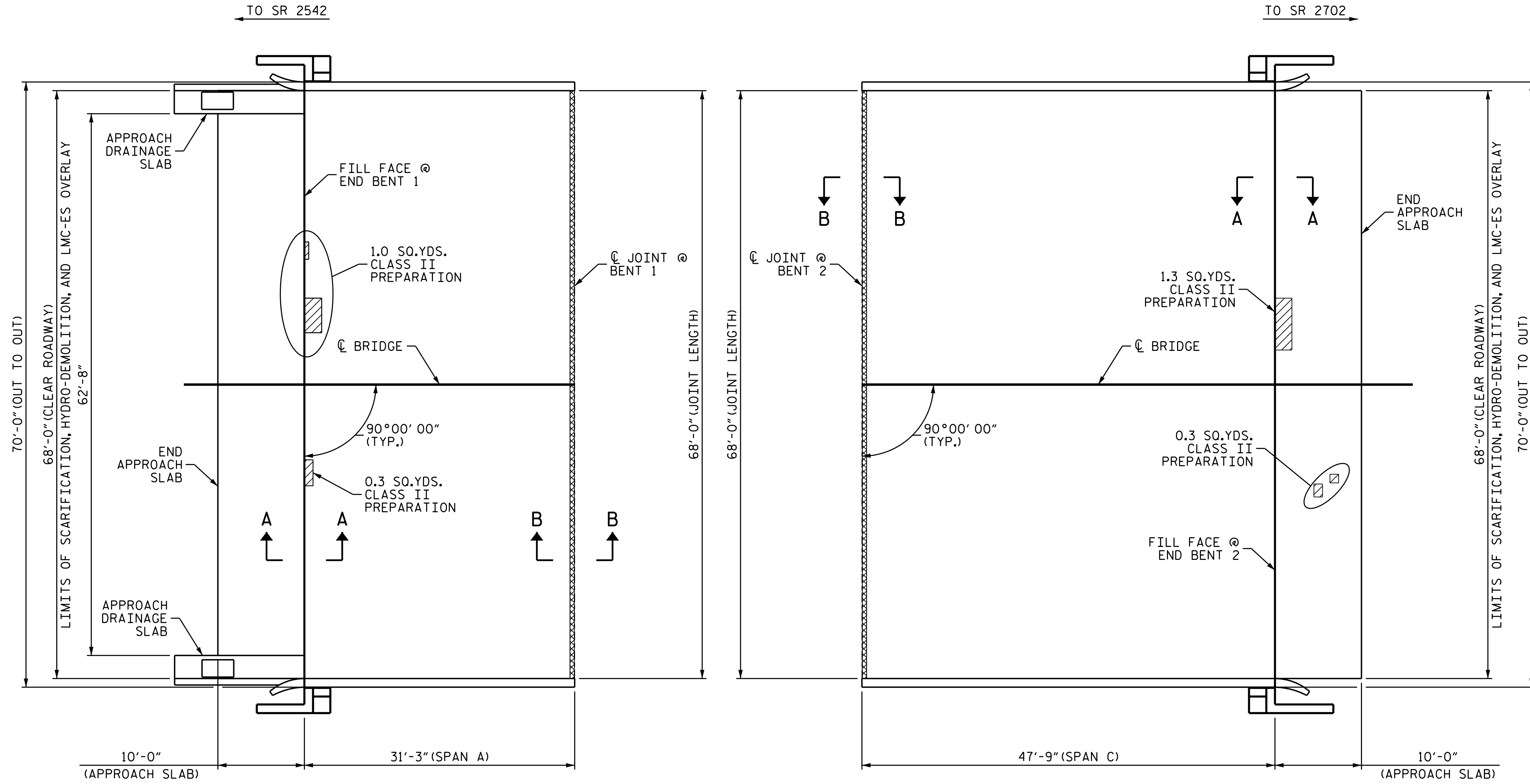
SPAN A
