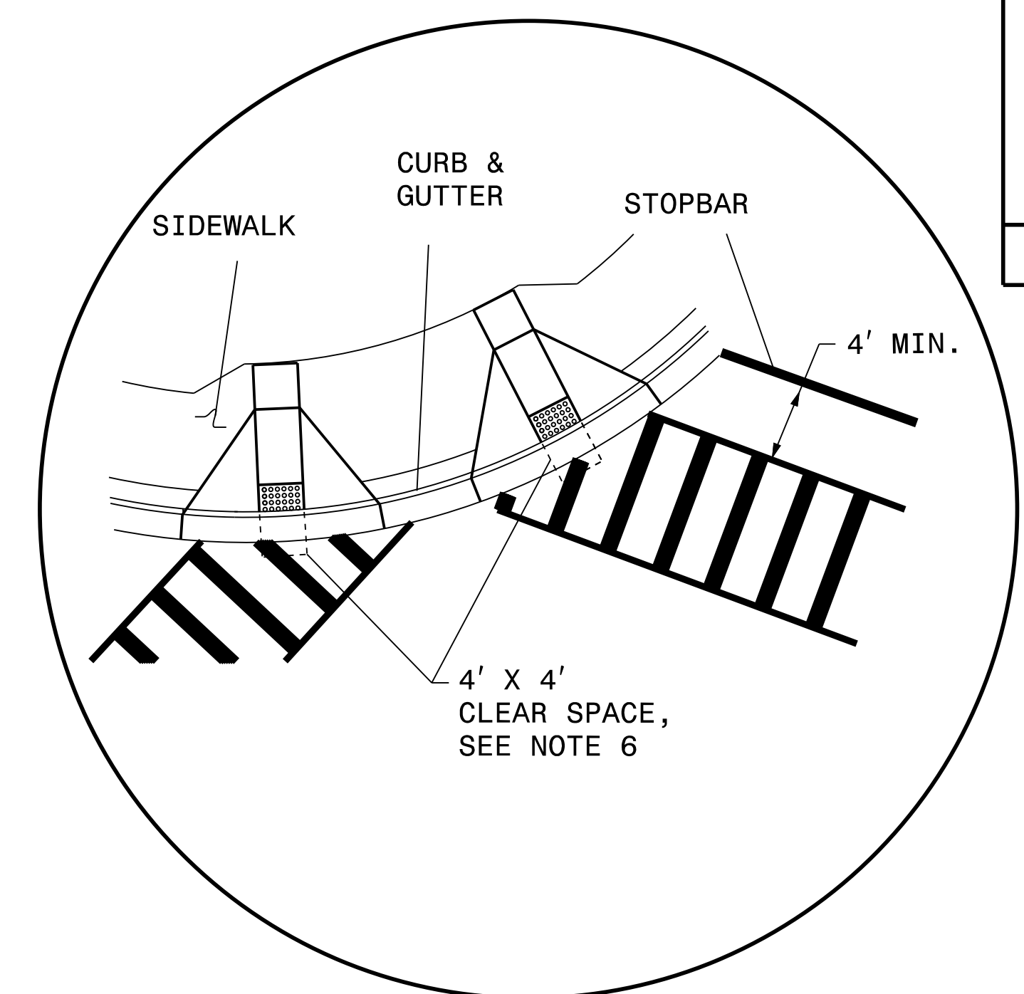
DETAIL 'A'- DUAL CURB RAMP
