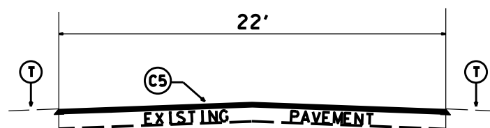
TYPICAL SECTION NO.9
