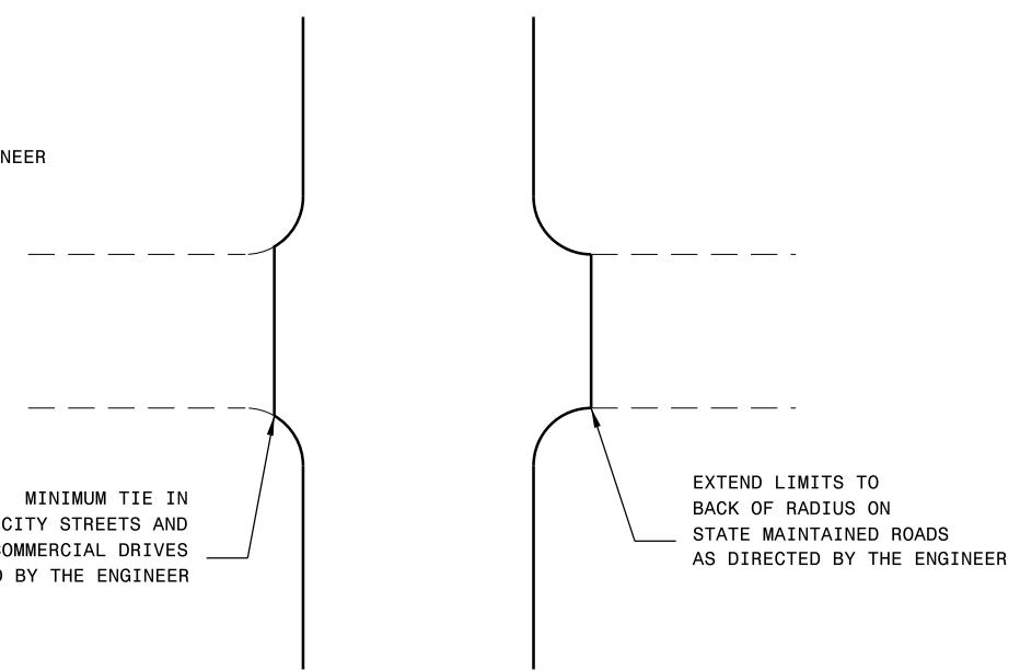
DETAIL OF PROJECT LIMITS AT UNSIGNALIZED Y LINES
