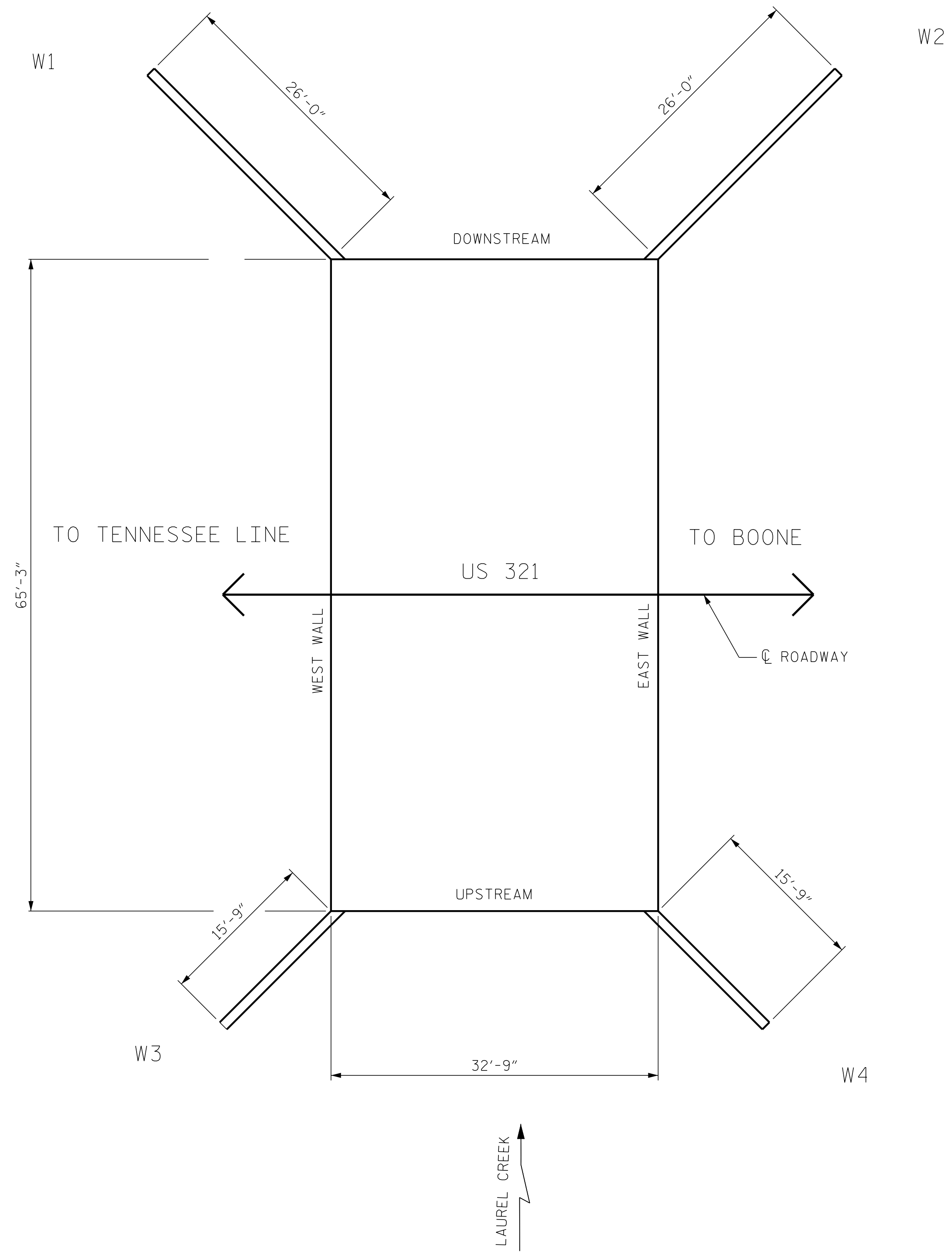
PLAN
