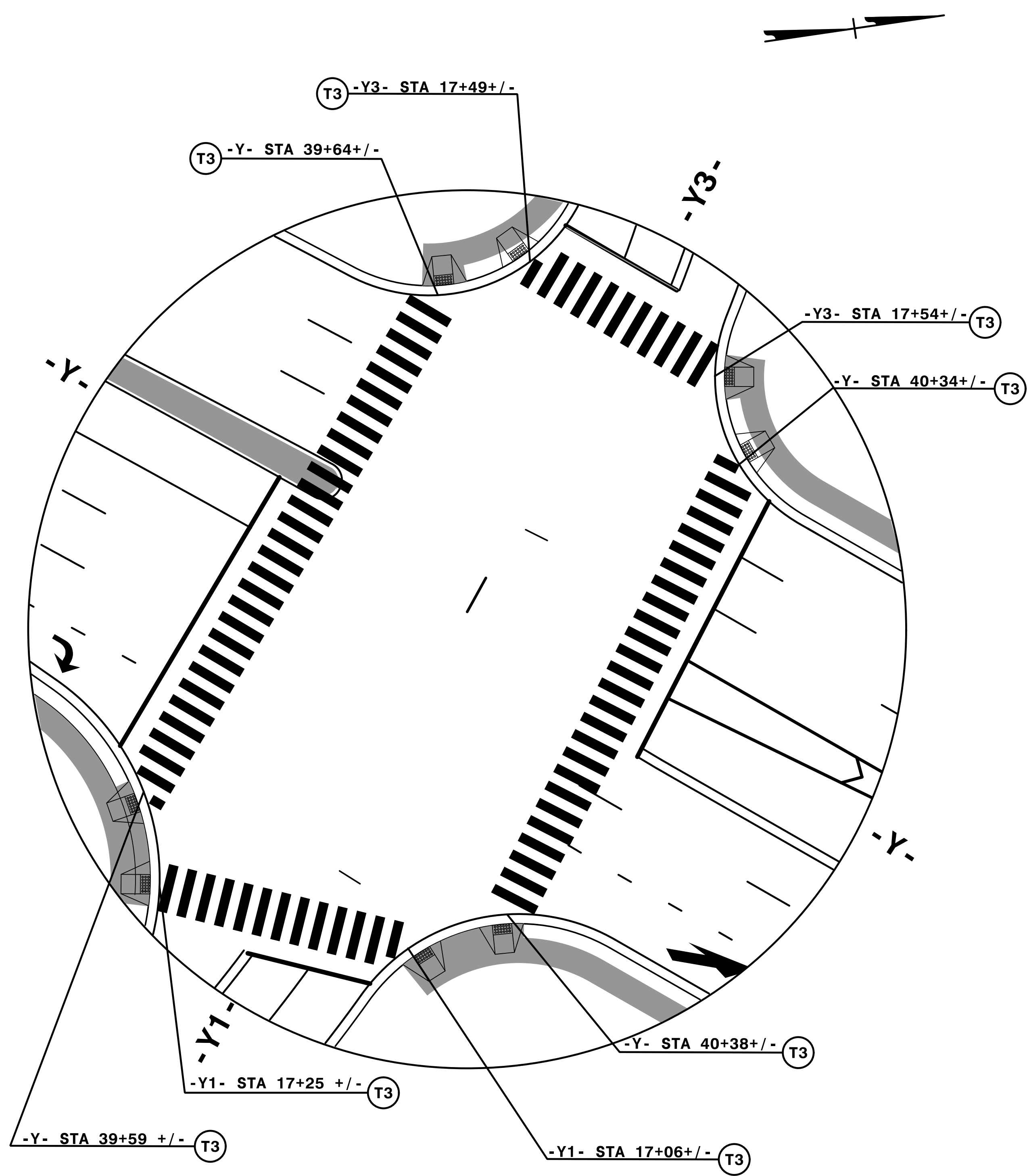
-Y- / -Y1- / -Y3- CROSSWALK LOCATIONS
