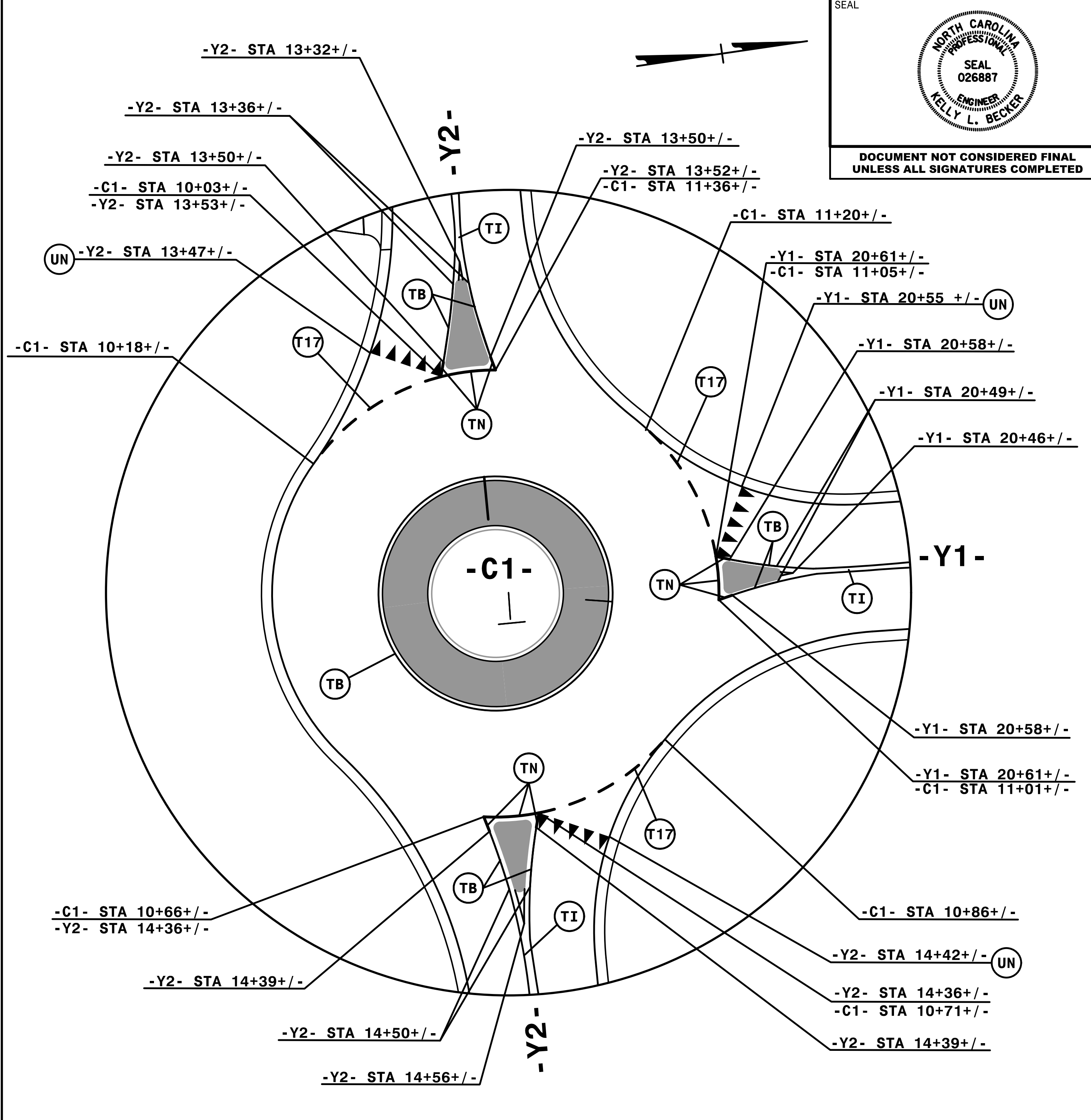
-Y1- / -Y2 ROUNDBOUT DETAIL
