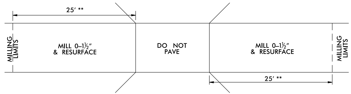
BRIDGE DRAWING USE FOR MAP #10, USE FOR BRIDGE #137 ** MILLING SHALL BE PAID FOR UNDER INCIDENTAL MILLING
