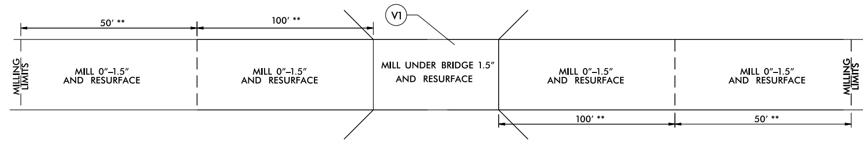
BRIDGE DRAWING FOR HWY# US 421 NB USE FOR MAP# 8, #42 USE FOR BRIDGE# 142, # 203 AND # 182
