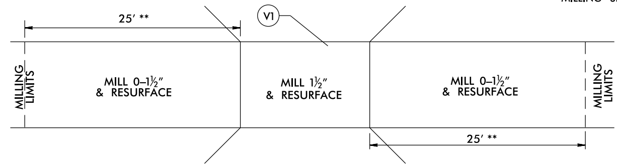
BRIDGE DRAWING USE FOR MAP #10, #15, #32, AND #34 USE FOR BRIDGE# 15, #342, #152, AND #151 ** MILLING SHALL BE PAID FOR UNDER INCIDENTAL MILLING
