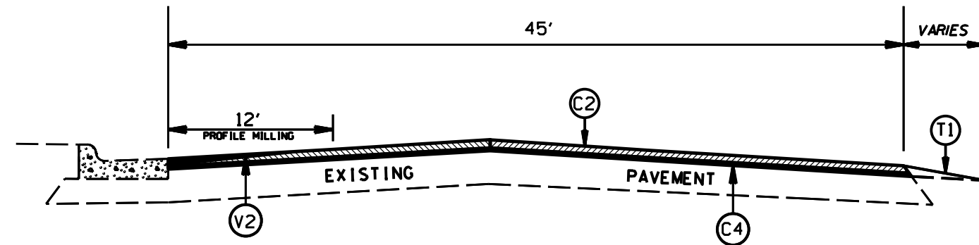
TYPICAL SECTION NO. 21
