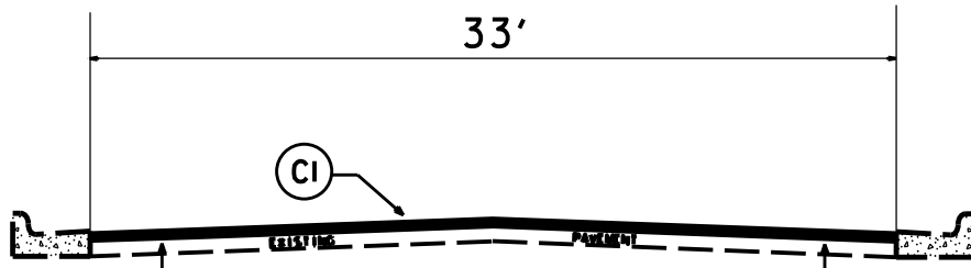
TYPICAL SECTION NO.4 Map: 54
