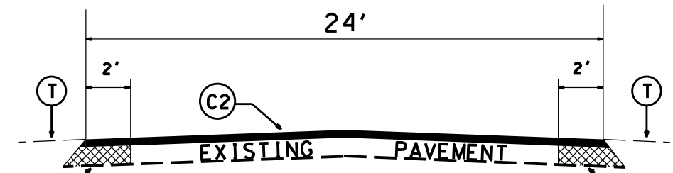
TYPICAL SECTION NO.8 Map 38
