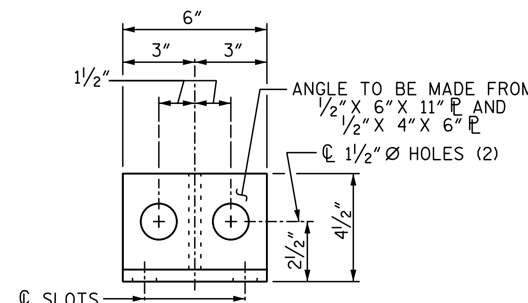
END VIEW
