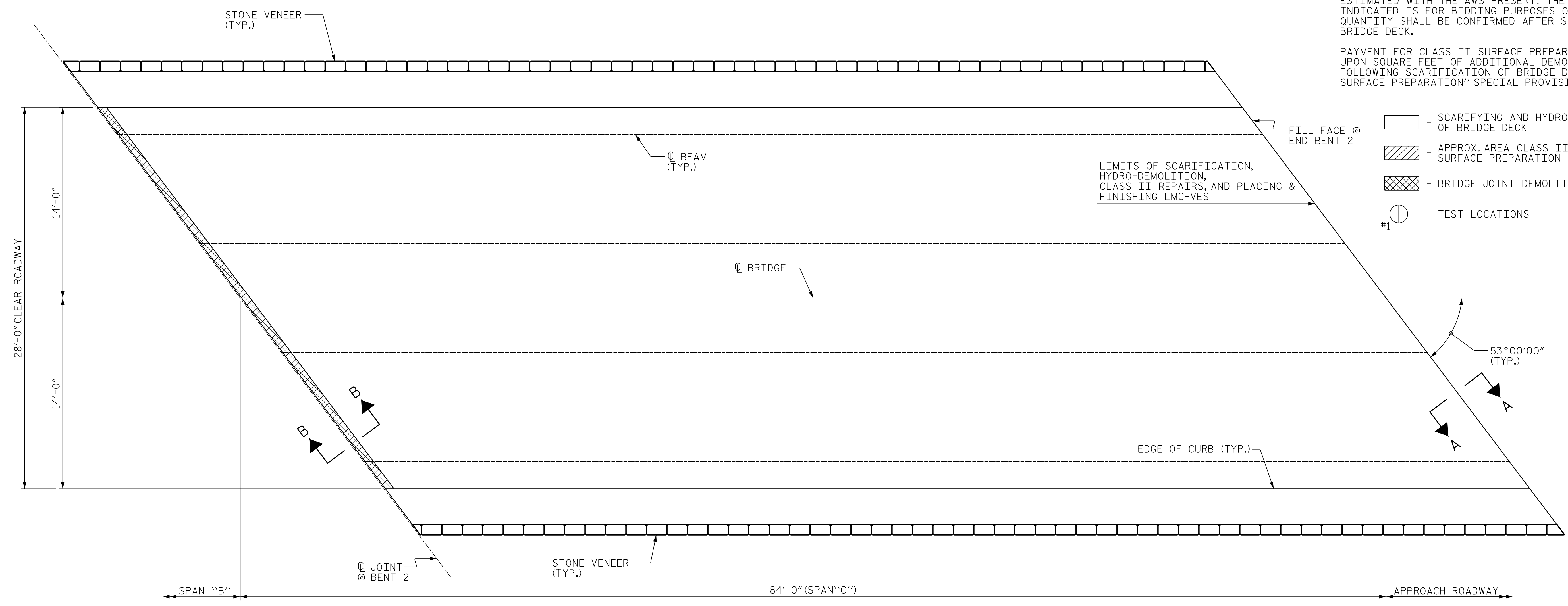
PLAN OF SPAN "C" (SEE SHEET NO. S-190 FOR SECTIONS A-A AND B-B)
