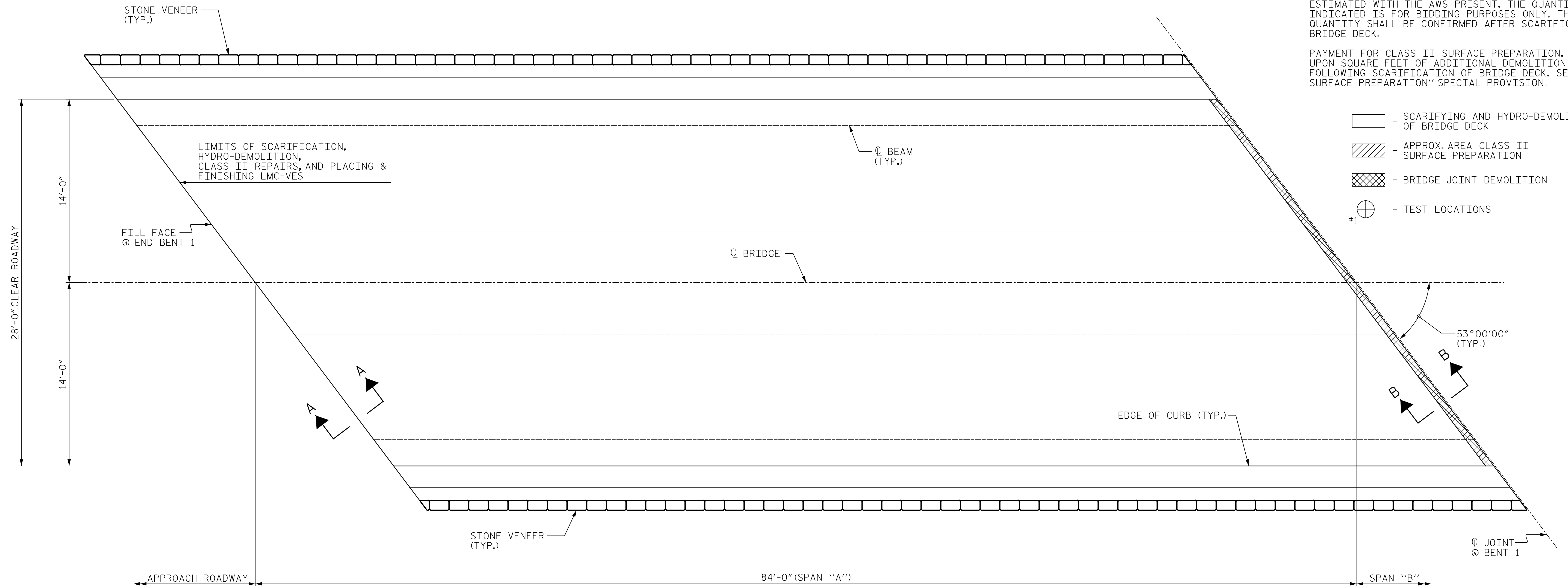
PLAN OF SPAN "A" (SEE SHEET NO. S-190 FOR SECTIONS A-A AND B-B)
