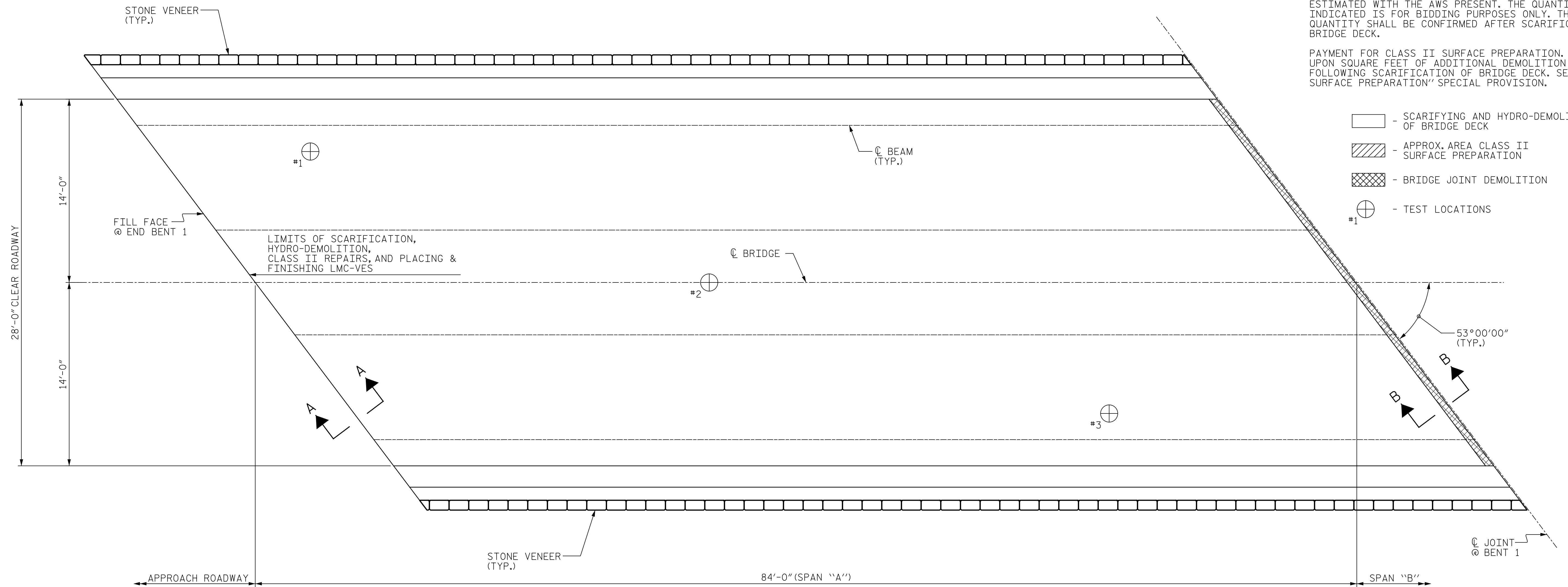
PLAN OF SPAN "A" (SEE SHEET NO. S-170 FOR SECTIONS A-A AND B-B)
