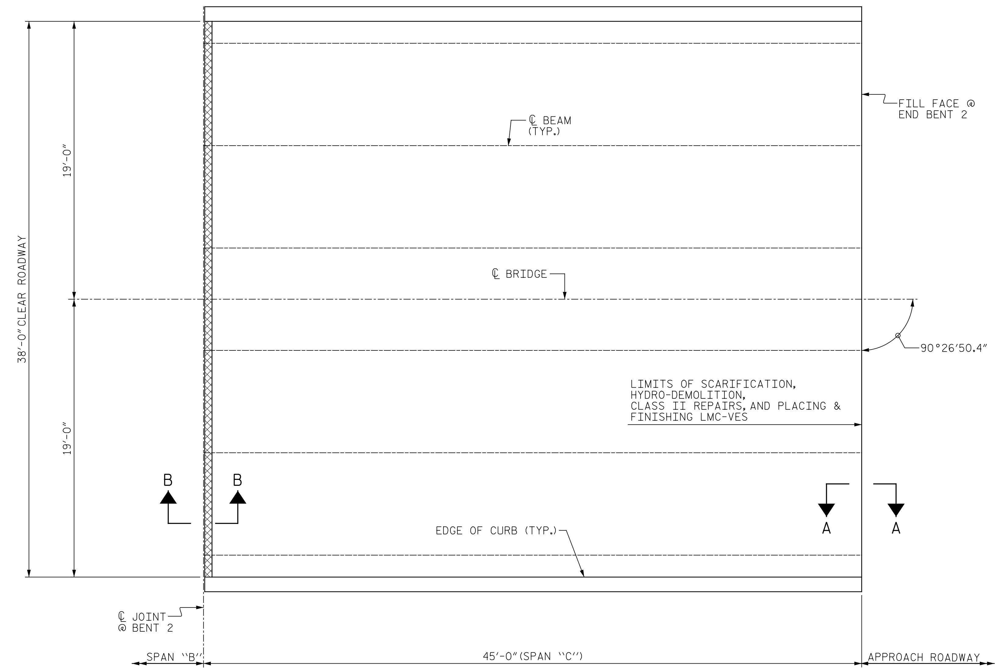
PLAN OF SPAN "C" (SEE SHEET NO. S-152 FOR SECTIONS A-A AND B-B)
