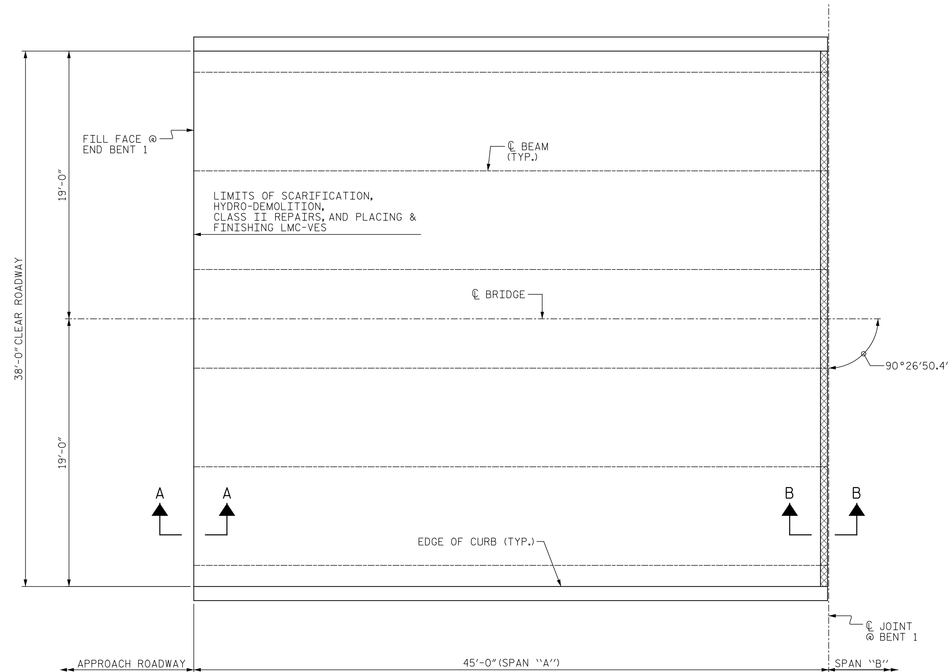
PLAN OF SPAN "A" (SEE SHEET NO. S-152 FOR SECTIONS A-A AND B-B)
