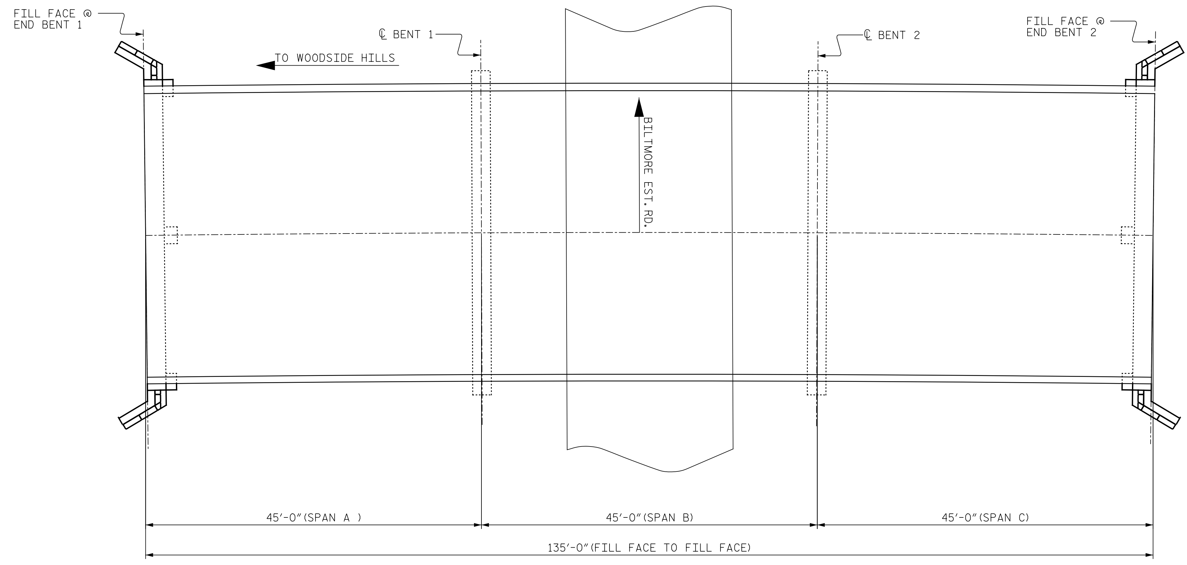
PLAN (PILES NOT SHOWN FOR CLARITY)
